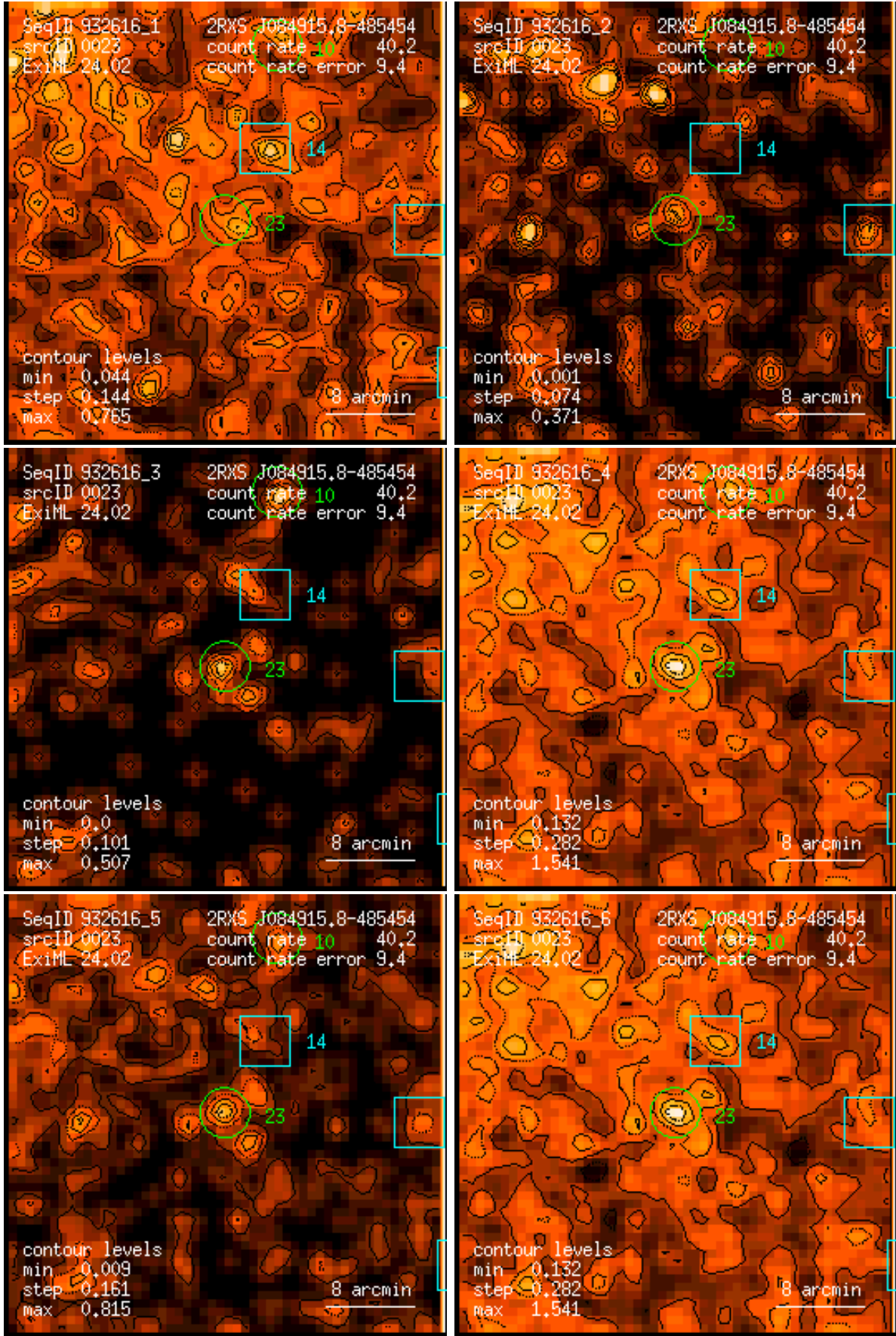
Figure 23: RASS 932616: detection 0023: band rate images, Gaussian filter: (1) PSPC channels 11 – 41, (2) 52 – 90, (3) 91 – 201, (4) 11 – 235, (5) 52 – 201, (6) 11 – 201. Broad band rates in counts/ks. Band rate contour levels in counts/ks/arcmin 2 .
