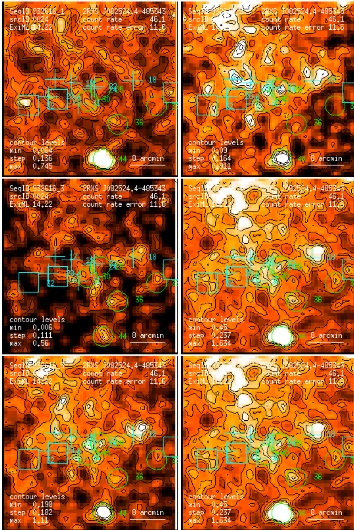
Figure 24: RASS 932616: detection 0024: band rate images, Gaussian filter: (1) PSPC channels 11 – 41, (2) 52 – 90, (3) 91 – 201, (4) 11 – 235, (5) 52 – 201, (6) 11 – 201. Broad band rates in counts/ks. Band rate contour levels in counts/ks/arcmin 2 .
