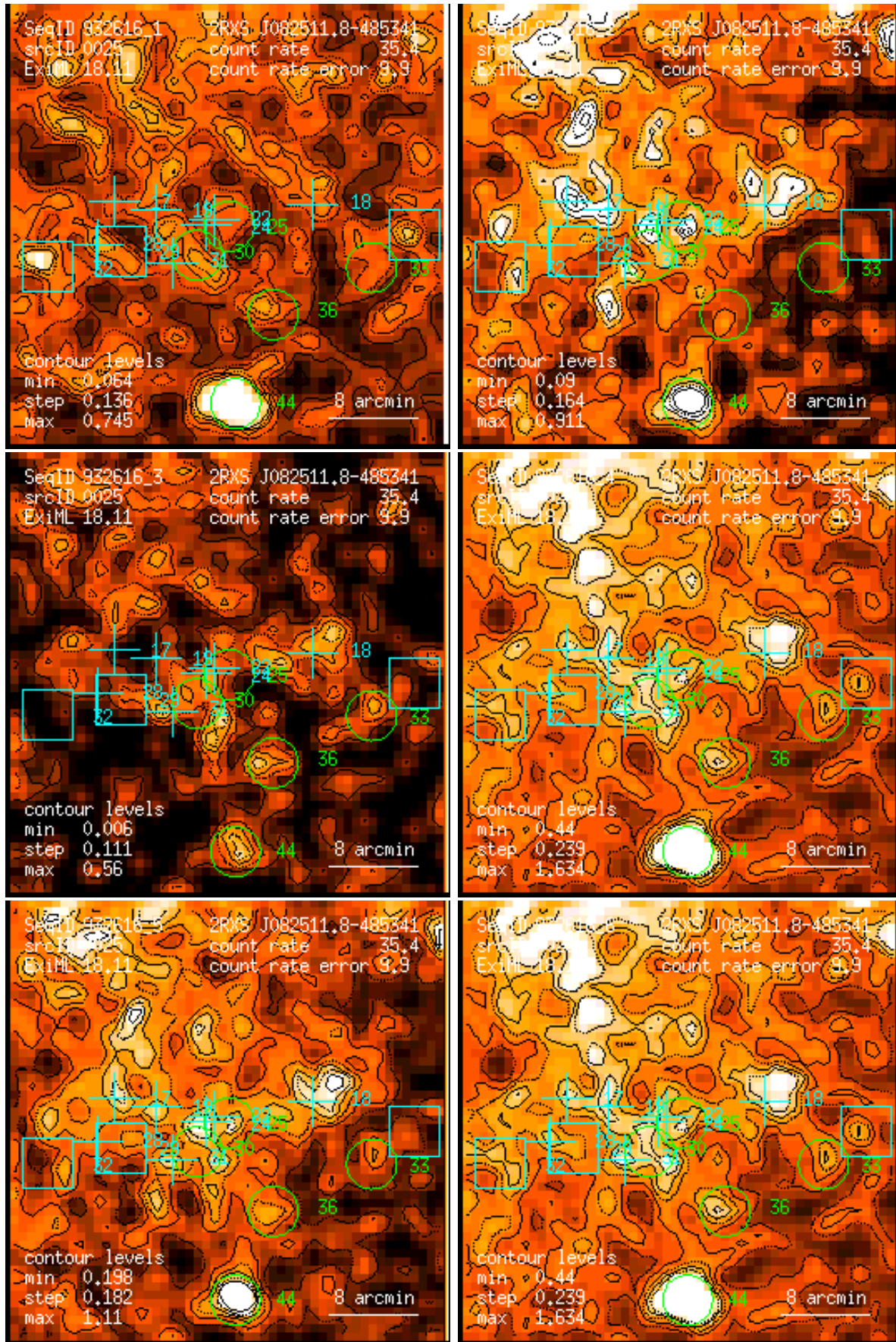
Figure 25: RASS 932616: detection 0025: band rate images, Gaussian filter: (1) PSPC channels 11 – 41, (2) 52 – 90, (3) 91 – 201, (4) 11 – 235, (5) 52 – 201, (6) 11 – 201. Broad band rates in counts/ks. Band rate contour levels in counts/ks/arcmin 2 .
