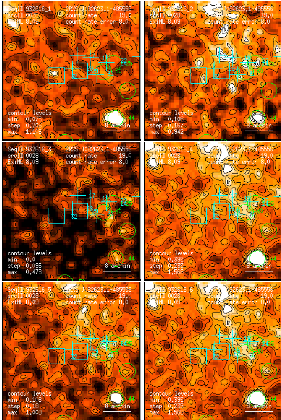
Figure 28: RASS 932616: detection 0028: band rate images, Gaussian filter: (1) PSPC channels 11 – 41, (2) 52 – 90, (3) 91 – 201, (4) 11 – 235, (5) 52 – 201, (6) 11 – 201. Broad band rates in counts/ks. Band rate contour levels in counts/ks/arcmin 2 .
