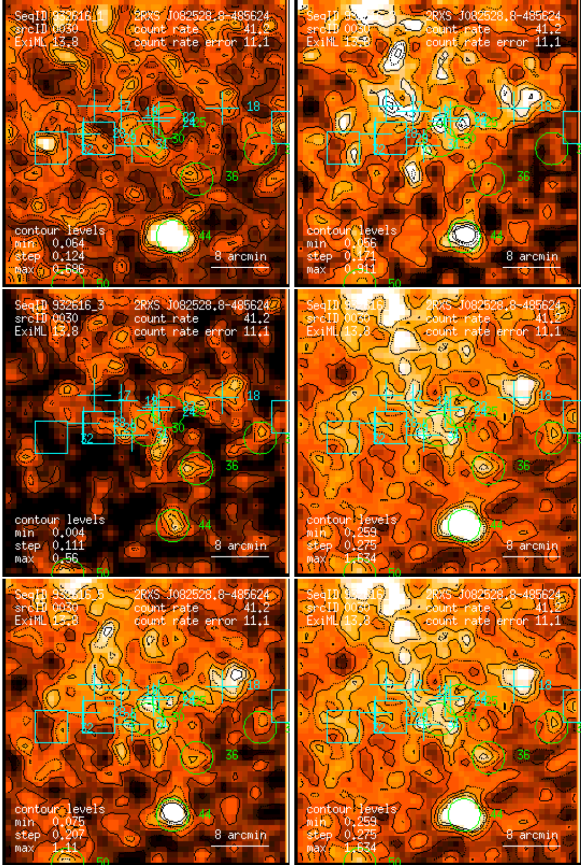
Figure 30: RASS 932616: detection 0030: band rate images, Gaussian filter: (1) PSPC channels 11 – 41, (2) 52 – 90, (3) 91 – 201, (4) 11 – 235, (5) 52 – 201, (6) 11 – 201. Broad band rates in counts/ks. Band rate contour levels in counts/ks/arcmin 2 .
