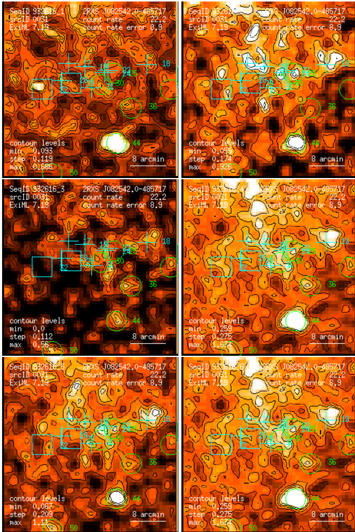
Figure 31: RASS 932616: detection 0031: band rate images, Gaussian filter: (1) PSPC channels 11 – 41, (2) 52 – 90, (3) 91 – 201, (4) 11 – 235, (5) 52 – 201, (6) 11 – 201. Broad band rates in counts/ks. Band rate contour levels in counts/ks/arcmin 2 .
