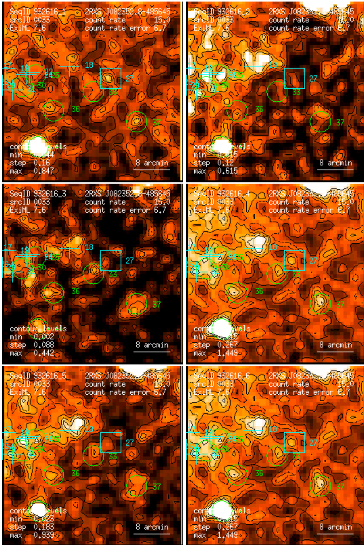
Figure 33: RASS 932616: detection 0033: band rate images, Gaussian filter: (1) PSPC channels 11 – 41, (2) 52 – 90, (3) 91 – 201, (4) 11 – 235, (5) 52 – 201, (6) 11 – 201. Broad band rates in counts/ks. Band rate contour levels in counts/ks/arcmin 2 .
