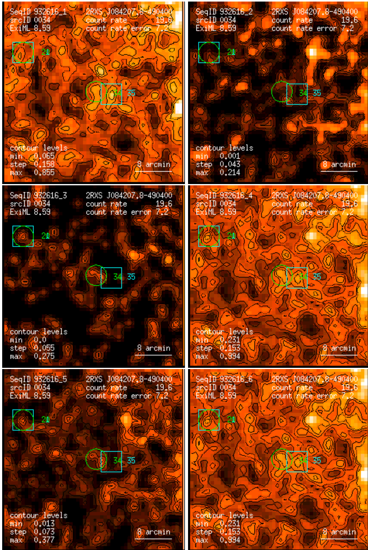
Figure 34: RASS 932616: detection 0034: band rate images, Gaussian filter: (1) PSPC channels 11 – 41, (2) 52 – 90, (3) 91 – 201, (4) 11 – 235, (5) 52 – 201, (6) 11 – 201. Broad band rates in counts/ks. Band rate contour levels in counts/ks/arcmin 2 .
