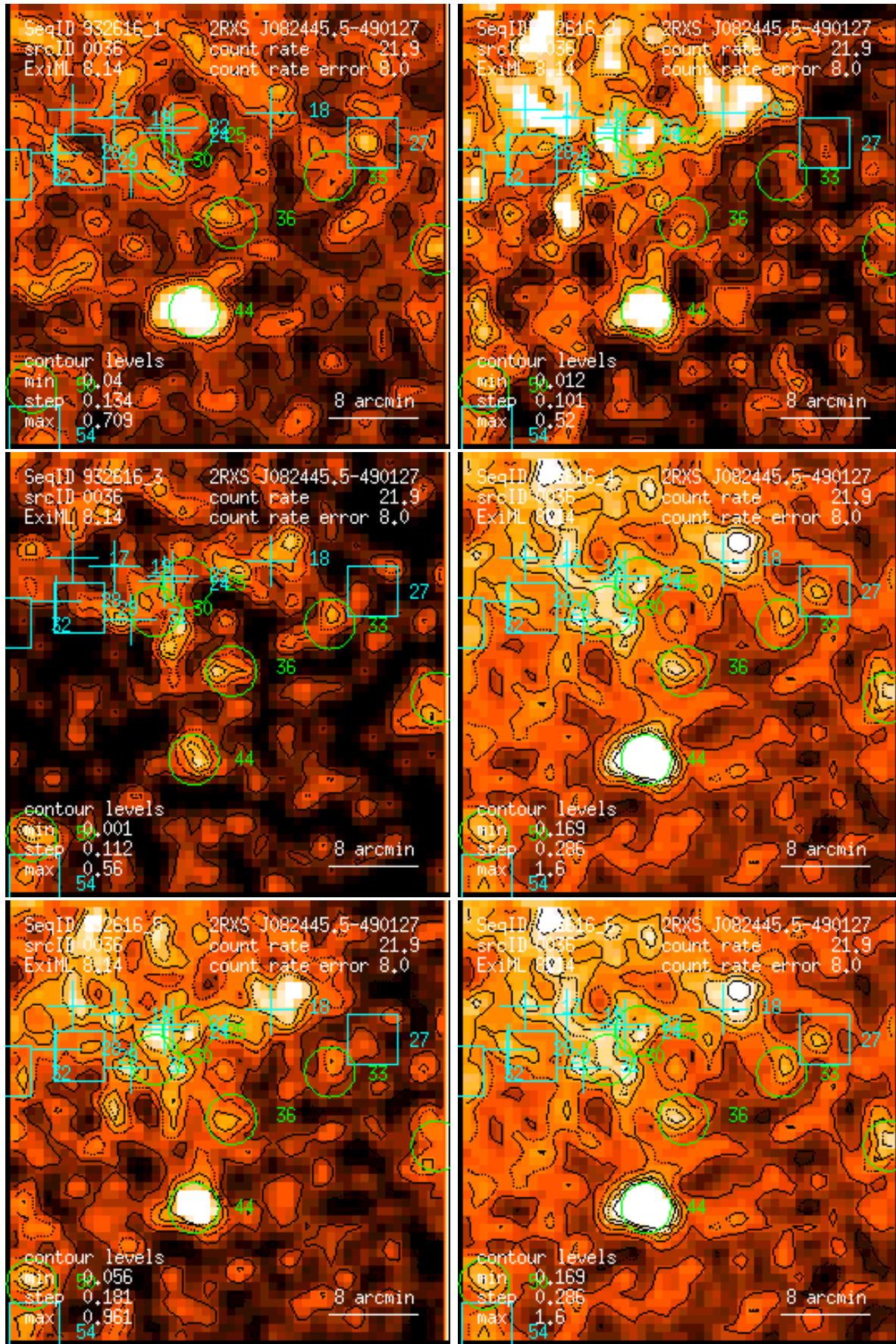
Figure 36: RASS 932616: detection 0036: band rate images, Gaussian filter: (1) PSPC channels 11 – 41, (2) 52 – 90, (3) 91 – 201, (4) 11 – 235, (5) 52 – 201, (6) 11 – 201. Broad band rates in counts/ks. Band rate contour levels in counts/ks/arcmin 2 .
