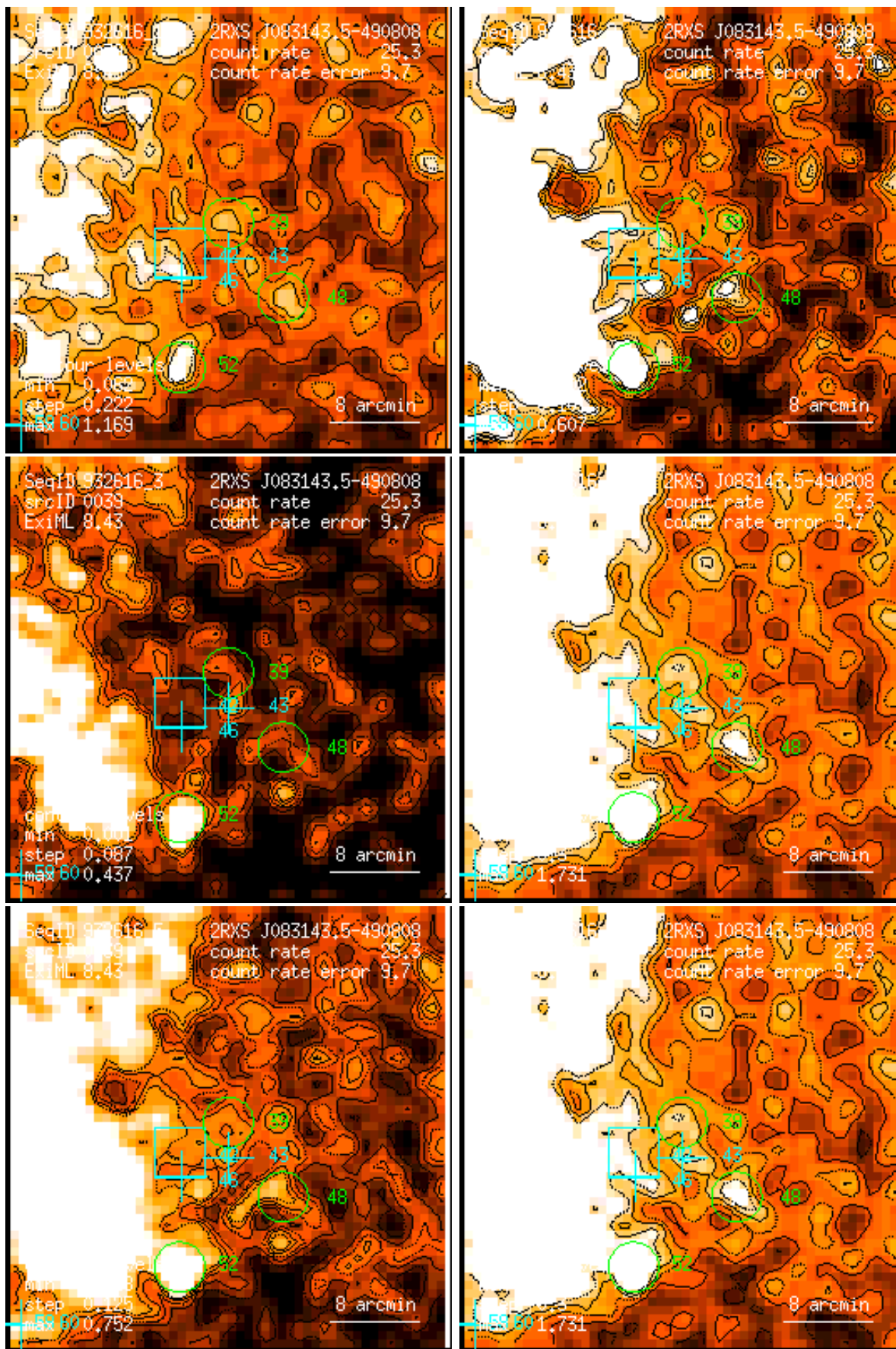
Figure 39: RASS 932616: detection 0039: band rate images, Gaussian filter: (1) PSPC channels 11 – 41, (2) 52 – 90, (3) 91 – 201, (4) 11 – 235, (5) 52 – 201, (6) 11 – 201. Broad band rates in counts/ks. Band rate contour levels in counts/ks/arcmin 2 .
