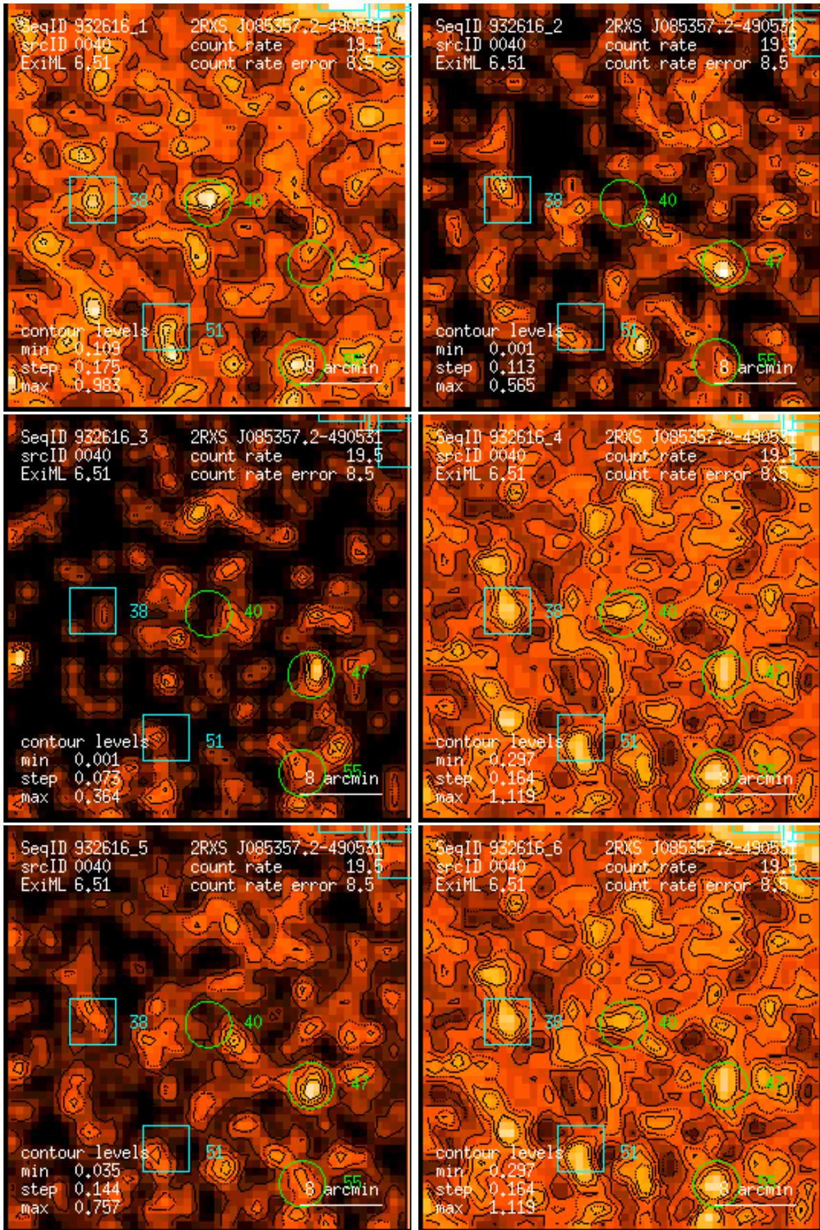
Figure 40: RASS 932616: detection 0040: band rate images, Gaussian filter: (1) PSPC channels 11 – 41, (2) 52 – 90, (3) 91 – 201, (4) 11 – 235, (5) 52 – 201, (6) 11 – 201. Broad band rates in counts/ks. Band rate contour levels in counts/ks/arcmin 2 .
