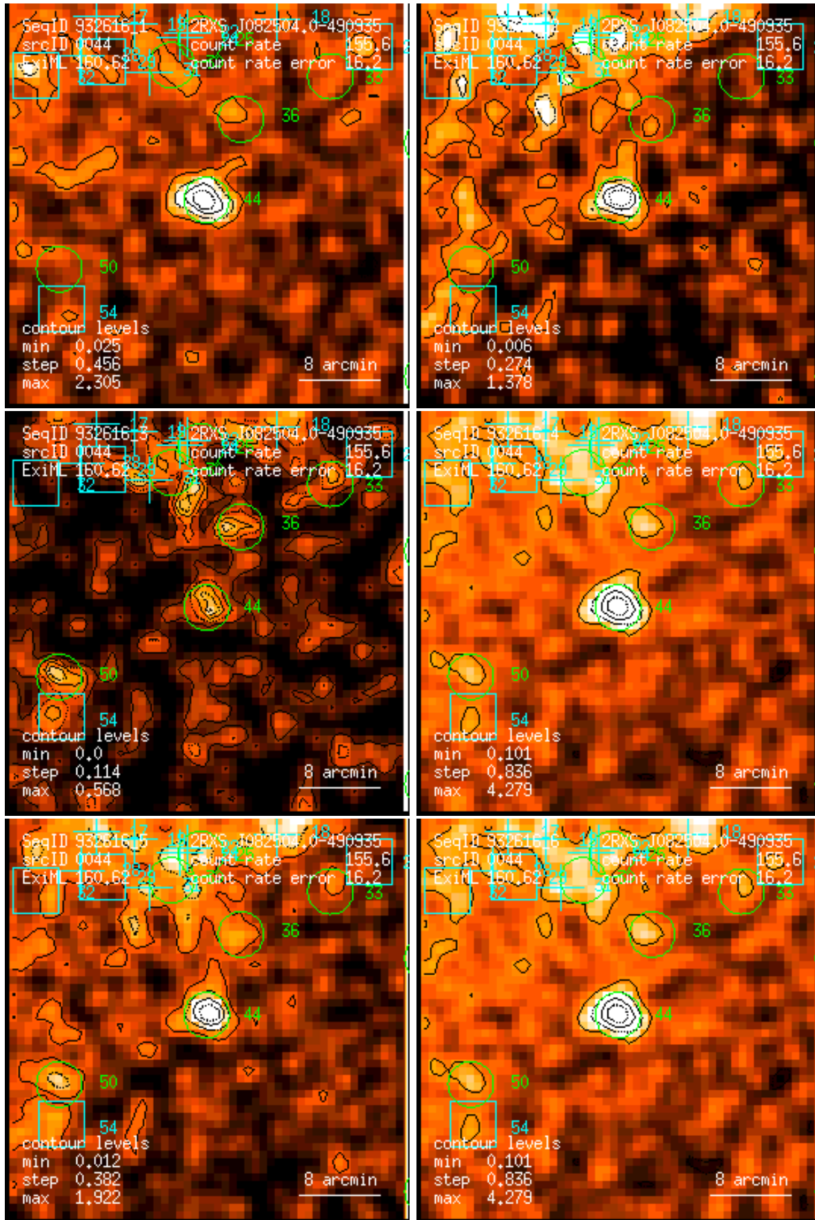
Figure 44: RASS 932616: detection 0044: band rate images, Gaussian filter: (1) PSPC channels 11 – 41, (2) 52 – 90, (3) 91 – 201, (4) 11 – 235, (5) 52 – 201, (6) 11 – 201. Broad band rates in counts/ks. Band rate contour levels in counts/ks/arcmin 2 .
