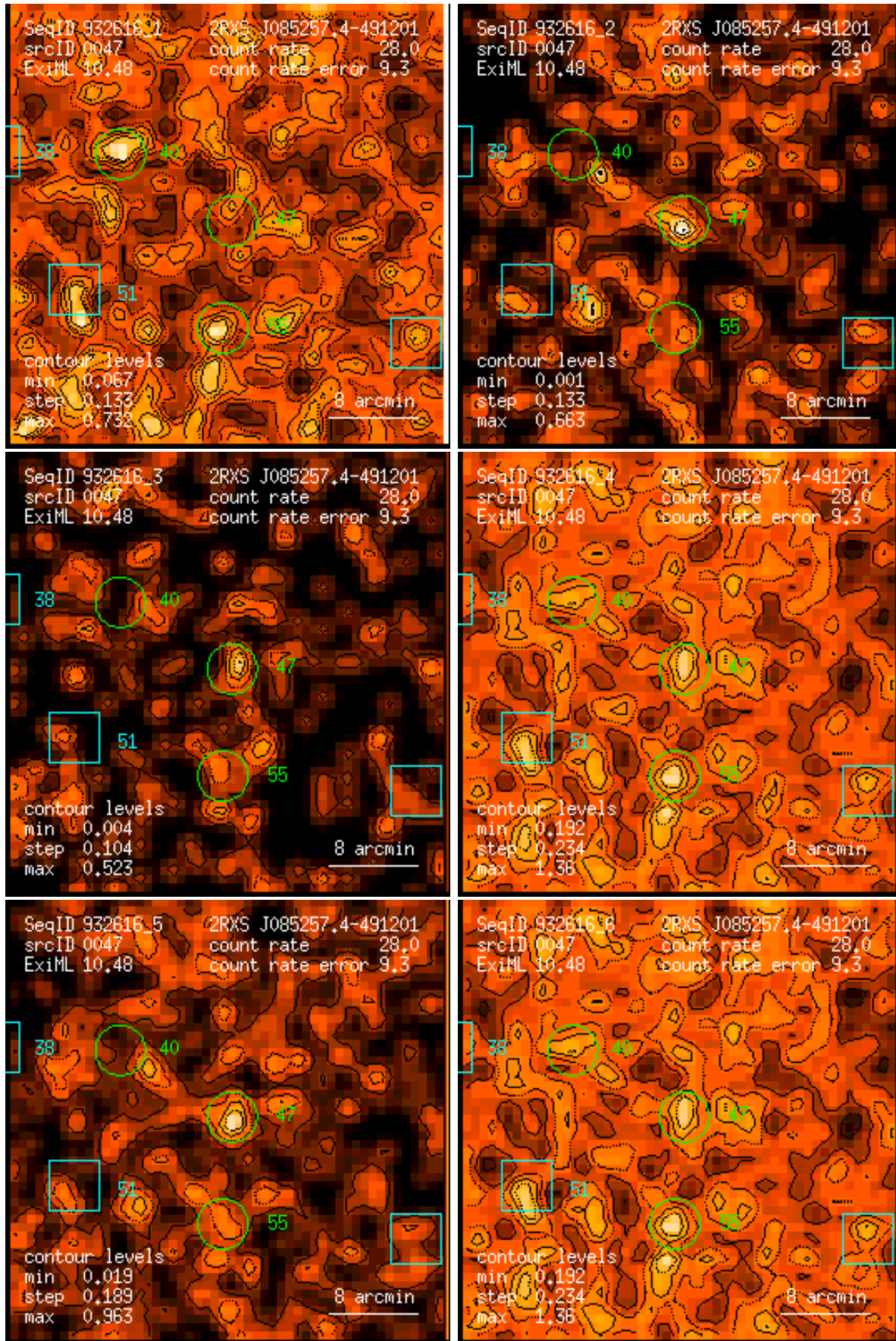
Figure 47: RASS 932616: detection 0047: band rate images, Gaussian filter: (1) PSPC channels 11 – 41, (2) 52 – 90, (3) 91 – 201, (4) 11 – 235, (5) 52 – 201, (6) 11 – 201. Broad band rates in counts/ks. Band rate contour levels in counts/ks/arcmin 2 .
