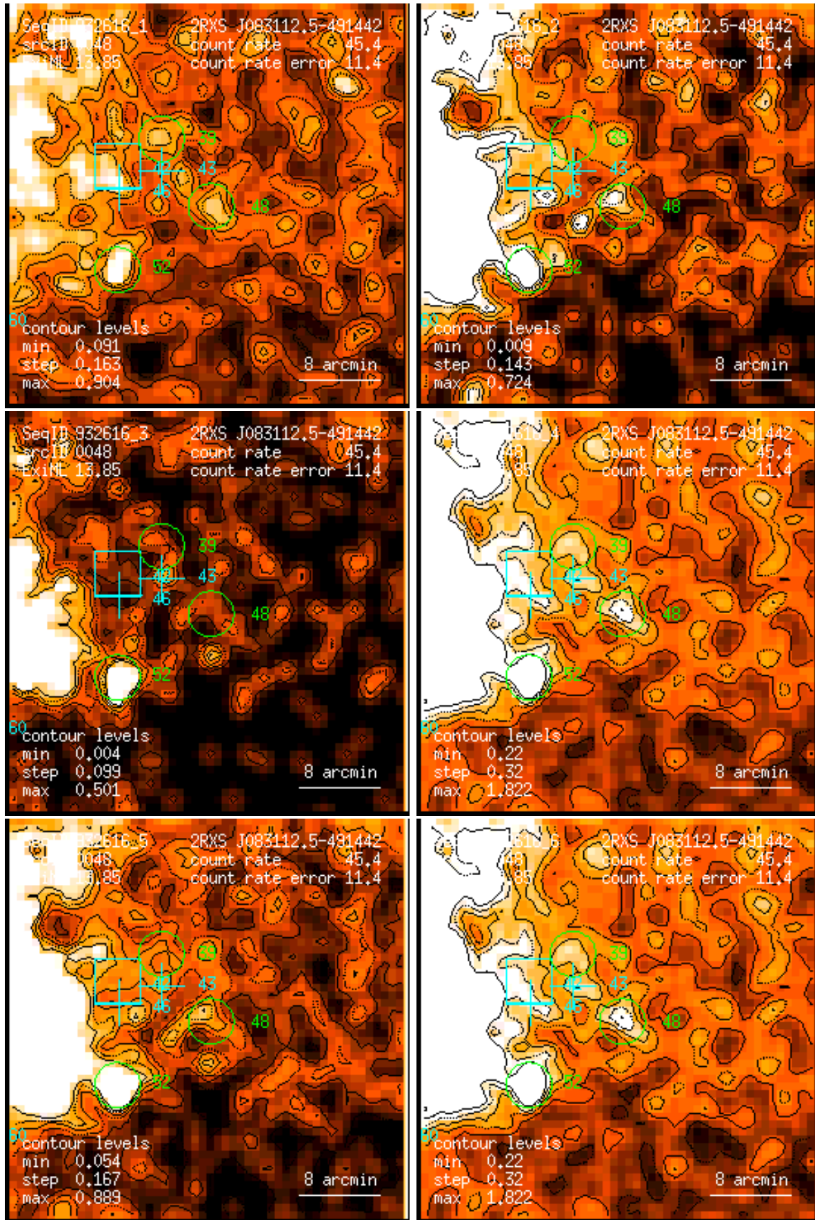
Figure 48: RASS 932616: detection 0048: band rate images, Gaussian filter: (1) PSPC channels 11 – 41, (2) 52 – 90, (3) 91 – 201, (4) 11 – 235, (5) 52 – 201, (6) 11 – 201. Broad band rates in counts/ks. Band rate contour levels in counts/ks/arcmin 2 .
