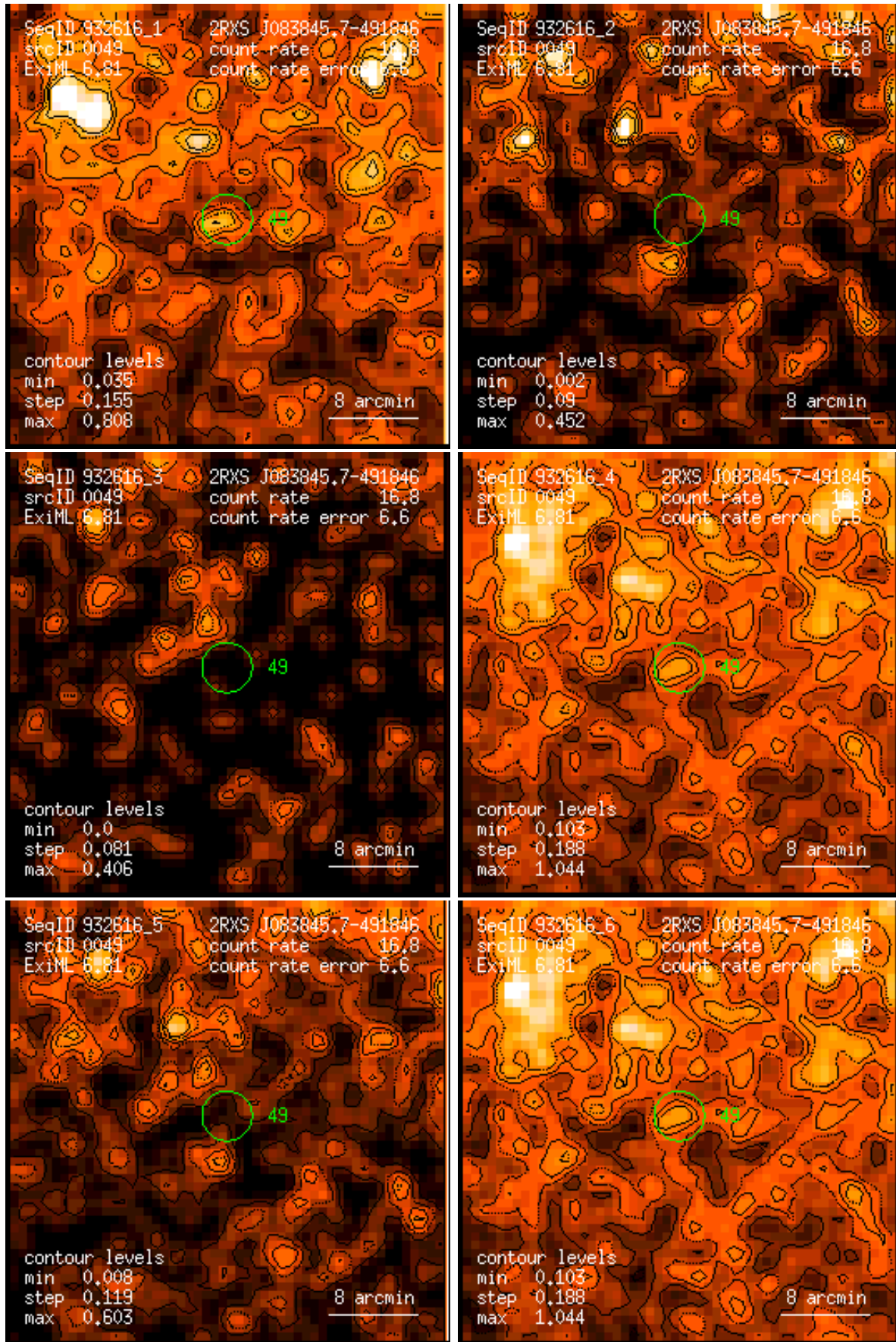
Figure 49: RASS 932616: detection 0049: band rate images, Gaussian filter: (1) PSPC channels 11 – 41, (2) 52 – 90, (3) 91 – 201, (4) 11 – 235, (5) 52 – 201, (6) 11 – 201. Broad band rates in counts/ks. Band rate contour levels in counts/ks/arcmin 2 .
