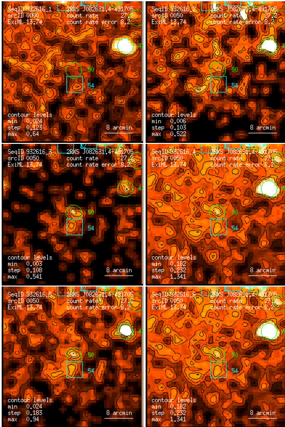
Figure 50: RASS 932616: detection 0050: band rate images, Gaussian filter: (1) PSPC channels 11 – 41, (2) 52 – 90, (3) 91 – 201, (4) 11 – 235, (5) 52 – 201, (6) 11 – 201. Broad band rates in counts/ks. Band rate contour levels in counts/ks/arcmin 2 .
