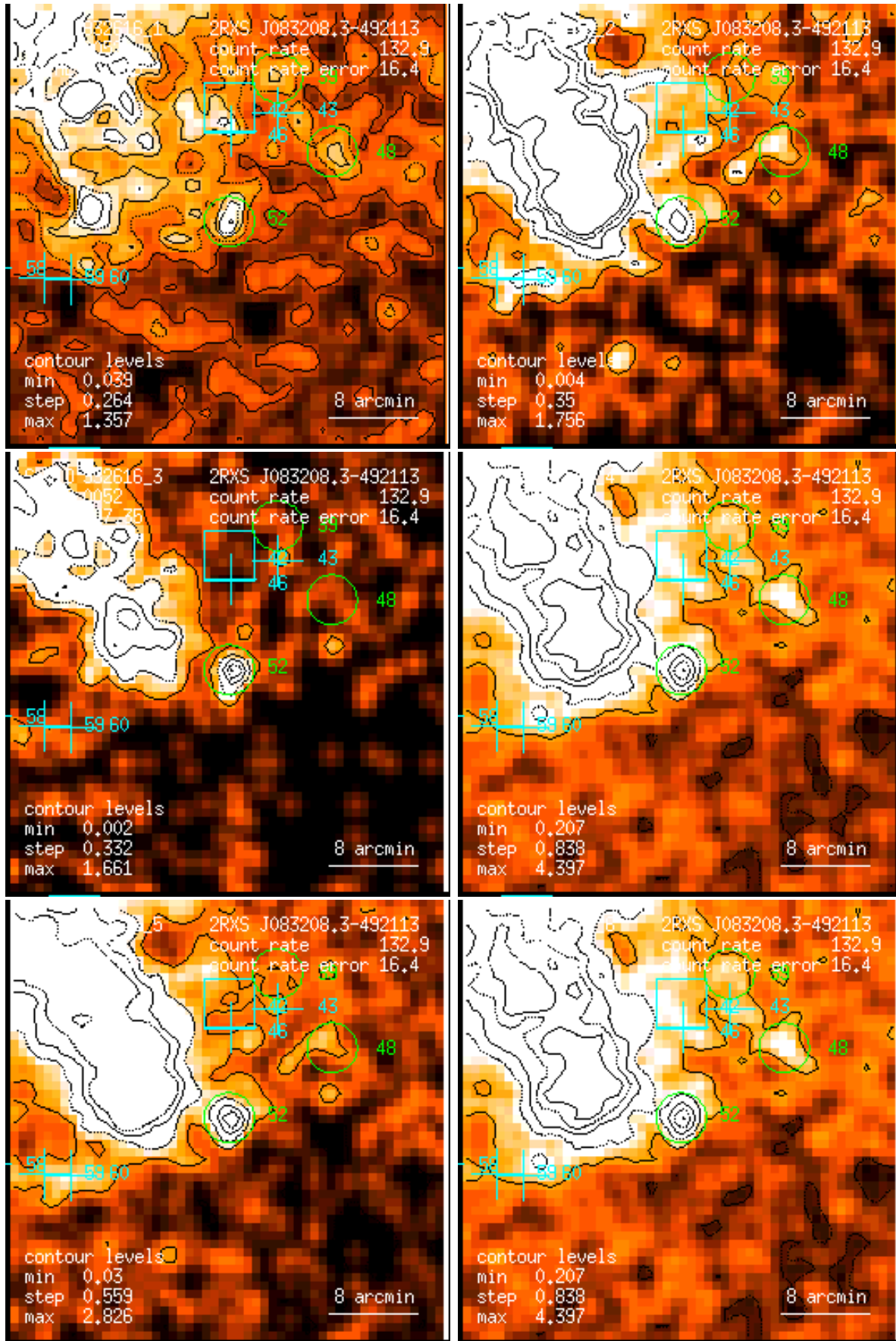
Figure 52: RASS 932616: detection 0052: band rate images, Gaussian filter: (1) PSPC channels 11 – 41, (2) 52 – 90, (3) 91 – 201, (4) 11 – 235, (5) 52 – 201, (6) 11 – 201. Broad band rates in counts/ks. Band rate contour levels in counts/ks/arcmin 2 .
