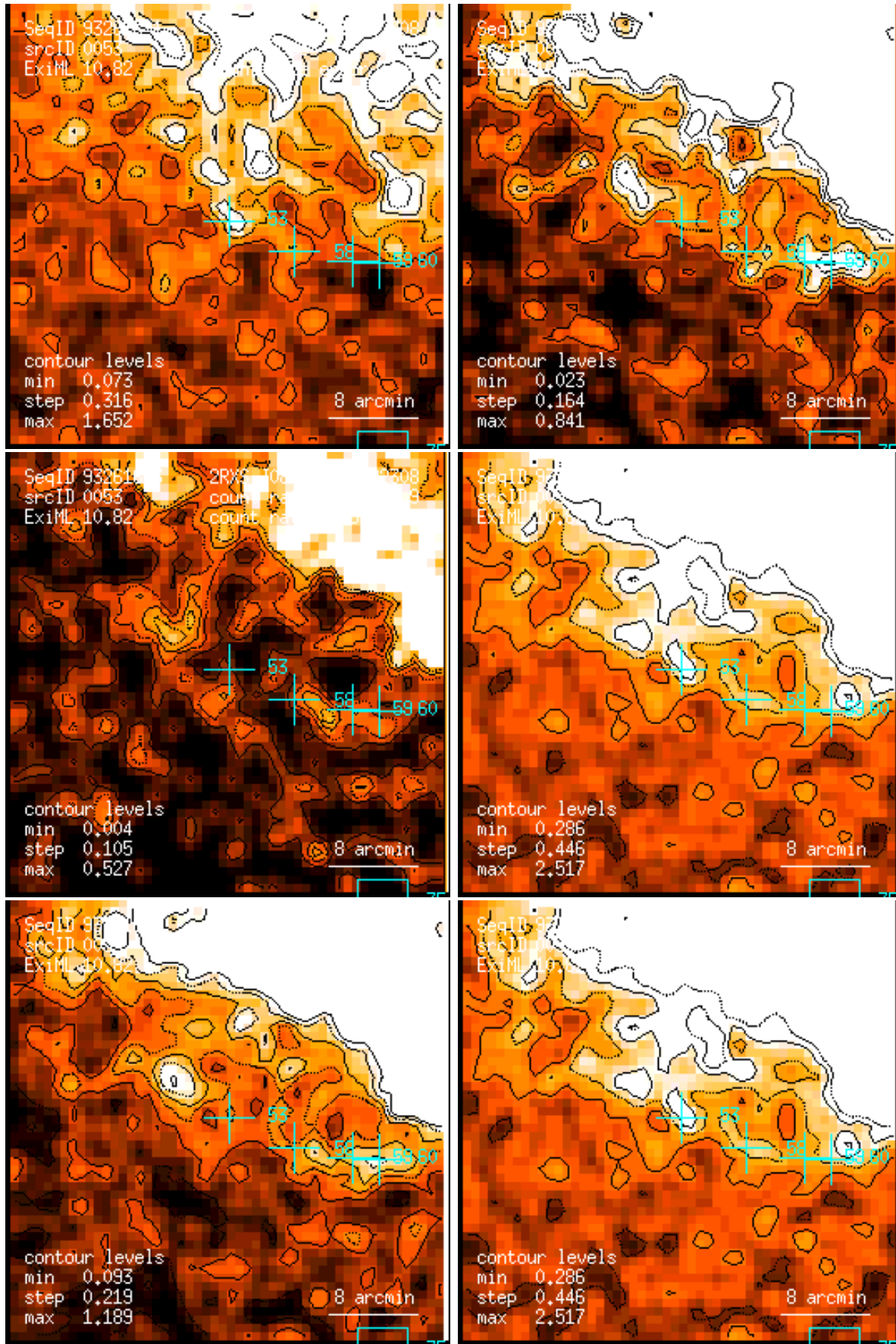
Figure 53: RASS 932616: detection 0053: band rate images, Gaussian filter: (1) PSPC channels 11 – 41, (2) 52 – 90, (3) 91 – 201, (4) 11 – 235, (5) 52 – 201, (6) 11 – 201. Broad band rates in counts/ks. Band rate contour levels in counts/ks/arcmin 2 .
