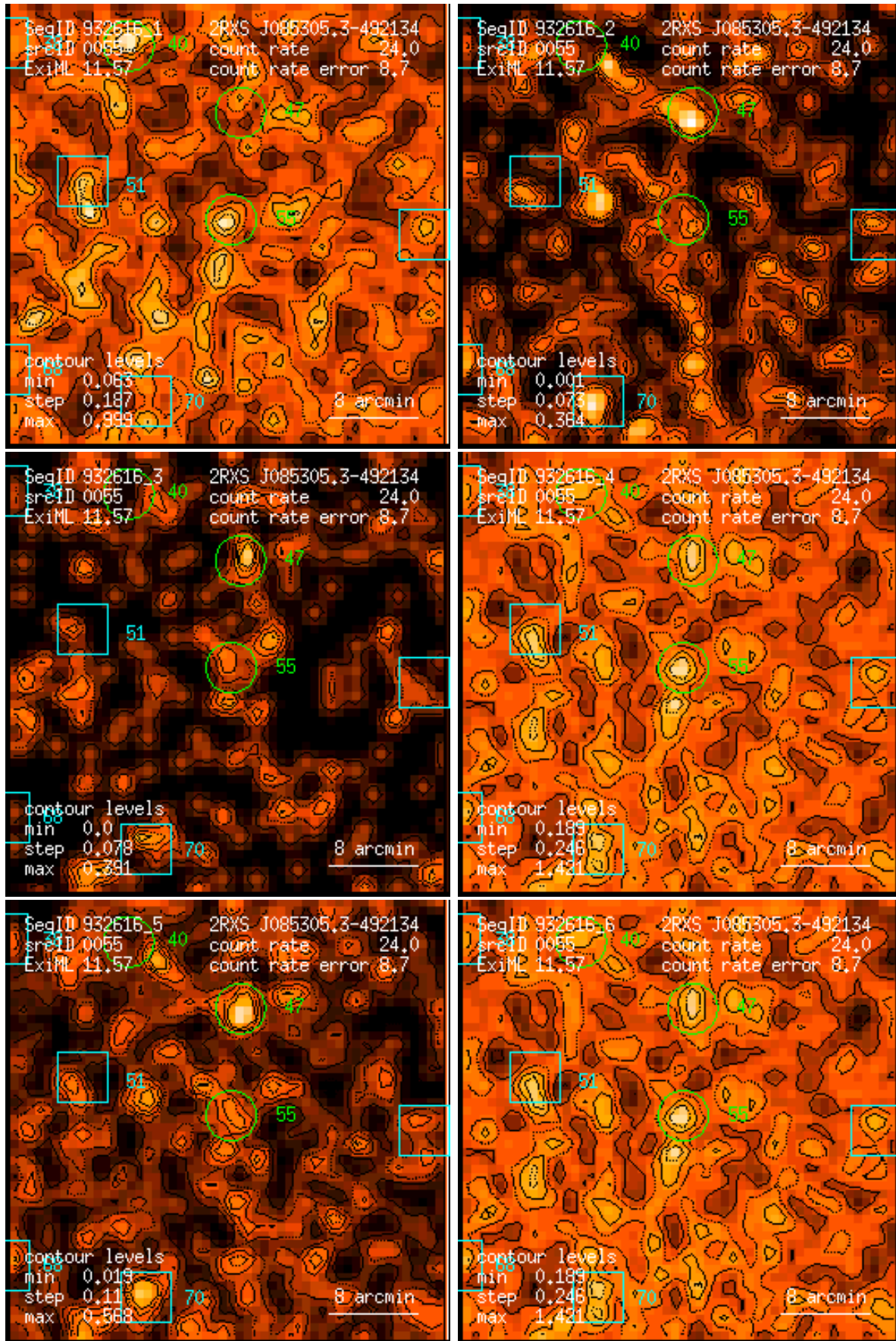
Figure 55: RASS 932616: detection 0055: band rate images, Gaussian filter: (1) PSPC channels 11 – 41, (2) 52 – 90, (3) 91 – 201, (4) 11 – 235, (5) 52 – 201, (6) 11 – 201. Broad band rates in counts/ks. Band rate contour levels in counts/ks/arcmin 2 .
