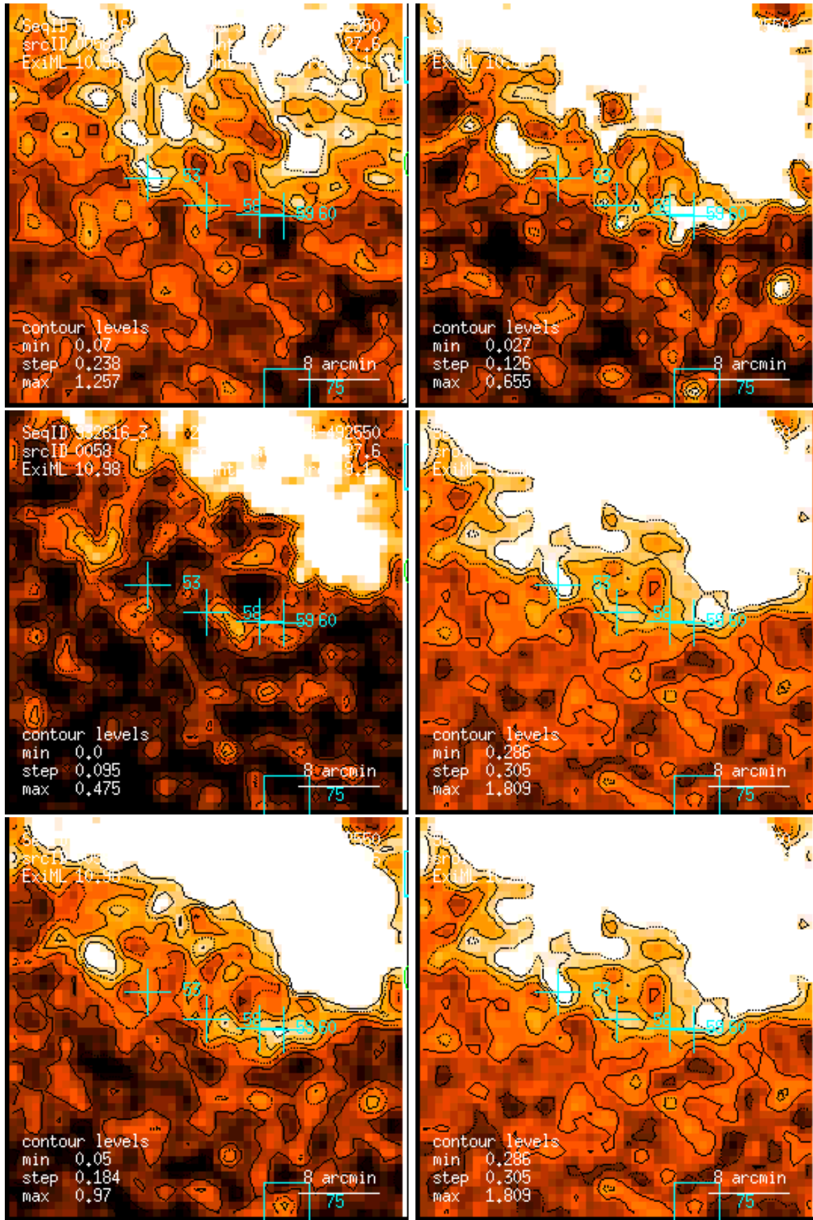
Figure 58: RASS 932616: detection 0058: band rate images, Gaussian filter: (1) PSPC channels 11 – 41, (2) 52 – 90, (3) 91 – 201, (4) 11 – 235, (5) 52 – 201, (6) 11 – 201. Broad band rates in counts/ks. Band rate contour levels in counts/ks/arcmin 2 .
