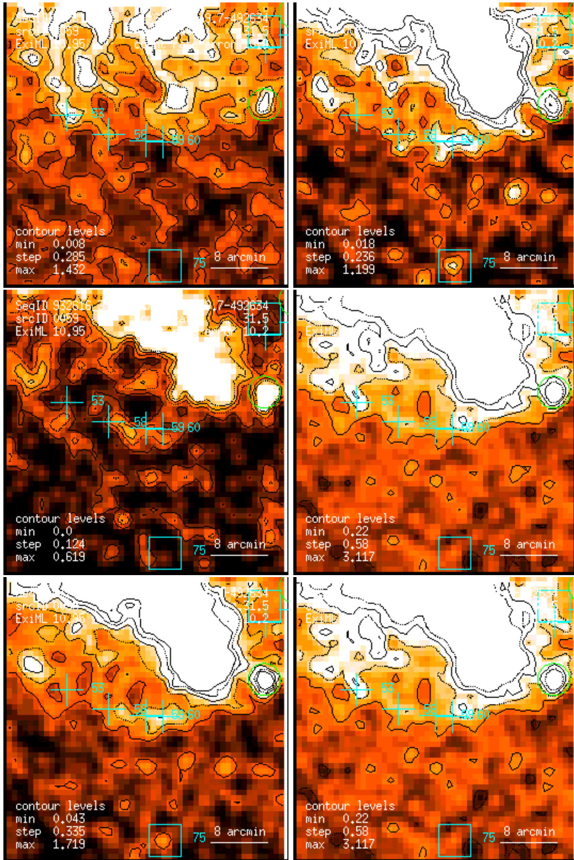
Figure 59: RASS 932616: detection 0059: band rate images, Gaussian filter: (1) PSPC channels 11 – 41, (2) 52 – 90, (3) 91 – 201, (4) 11 – 235, (5) 52 – 201, (6) 11 – 201. Broad band rates in counts/ks. Band rate contour levels in counts/ks/arcmin 2 .
