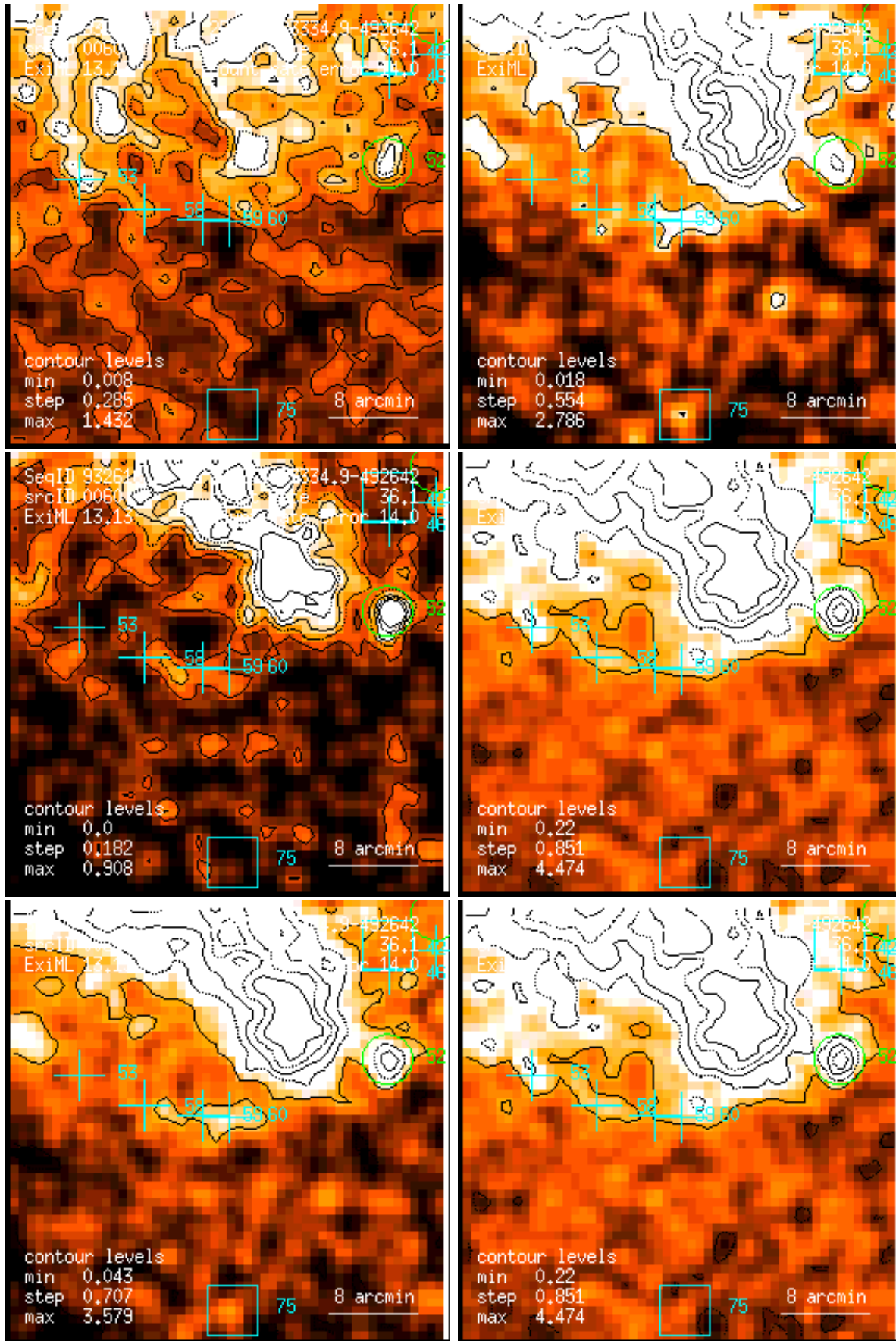
Figure 60: RASS 932616: detection 0060: band rate images, Gaussian filter: (1) PSPC channels 11 – 41, (2) 52 – 90, (3) 91 – 201, (4) 11 – 235, (5) 52 – 201, (6) 11 – 201. Broad band rates in counts/ks. Band rate contour levels in counts/ks/arcmin 2 .
