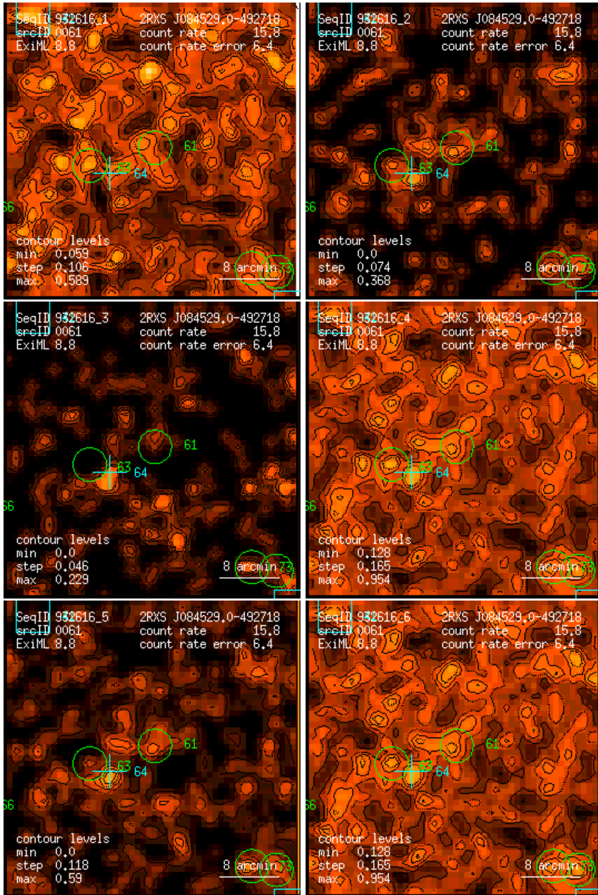
Figure 61: RASS 932616: detection 0061: band rate images, Gaussian filter: (1) PSPC channels 11 – 41, (2) 52 – 90, (3) 91 – 201, (4) 11 – 235, (5) 52 – 201, (6) 11 – 201. Broad band rates in counts/ks. Band rate contour levels in counts/ks/arcmin 2 .
