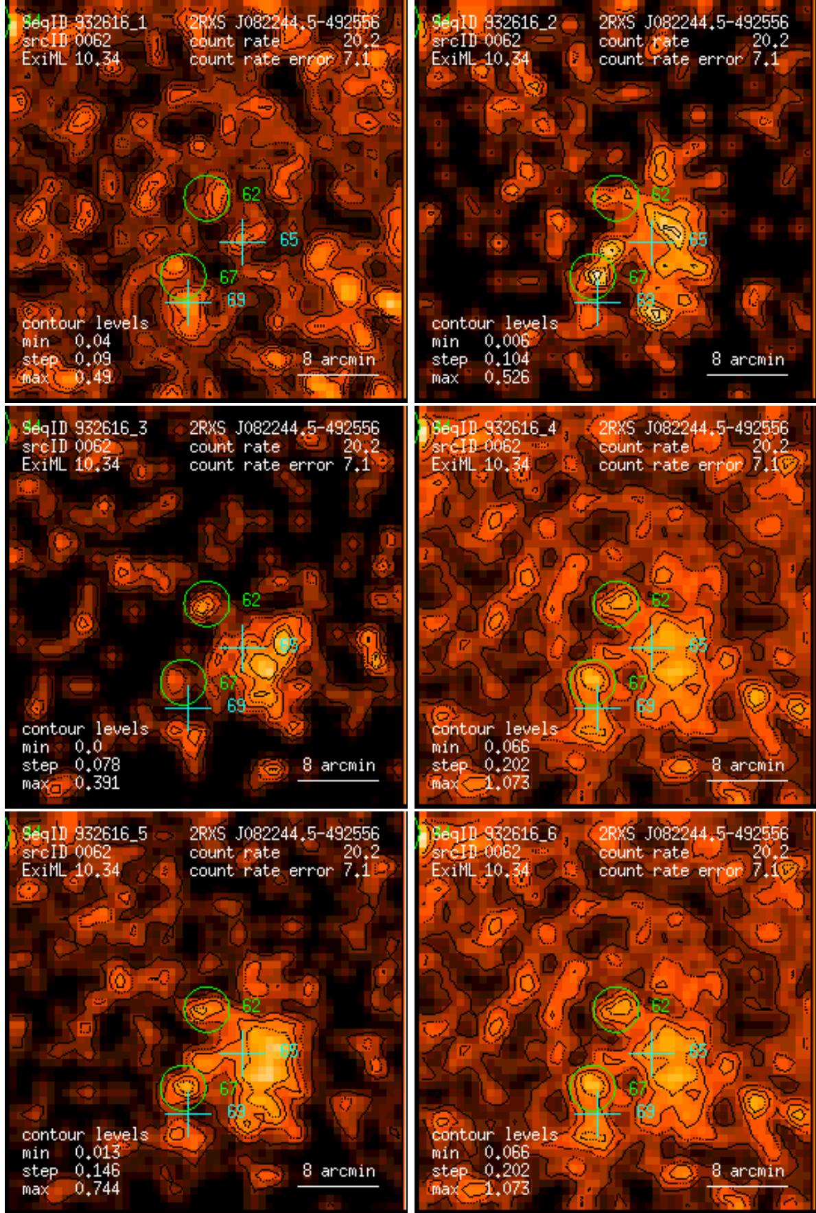
Figure 62: RASS 932616: detection 0062: band rate images, Gaussian filter: (1) PSPC channels 11 – 41, (2) 52 – 90, (3) 91 – 201, (4) 11 – 235, (5) 52 – 201, (6) 11 – 201. Broad band rates in counts/ks. Band rate contour levels in counts/ks/arcmin 2 .
