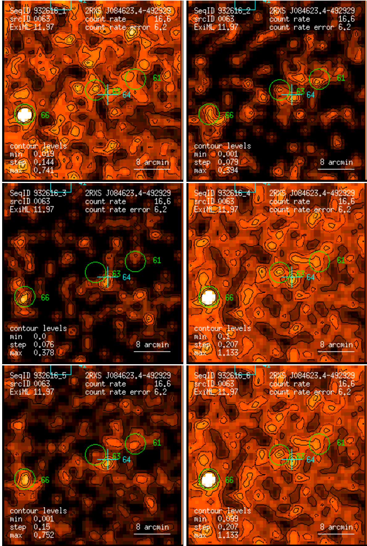
Figure 63: RASS 932616: detection 0063: band rate images, Gaussian filter: (1) PSPC channels 11 – 41, (2) 52 – 90, (3) 91 – 201, (4) 11 – 235, (5) 52 – 201, (6) 11 – 201. Broad band rates in counts/ks. Band rate contour levels in counts/ks/arcmin 2 .
