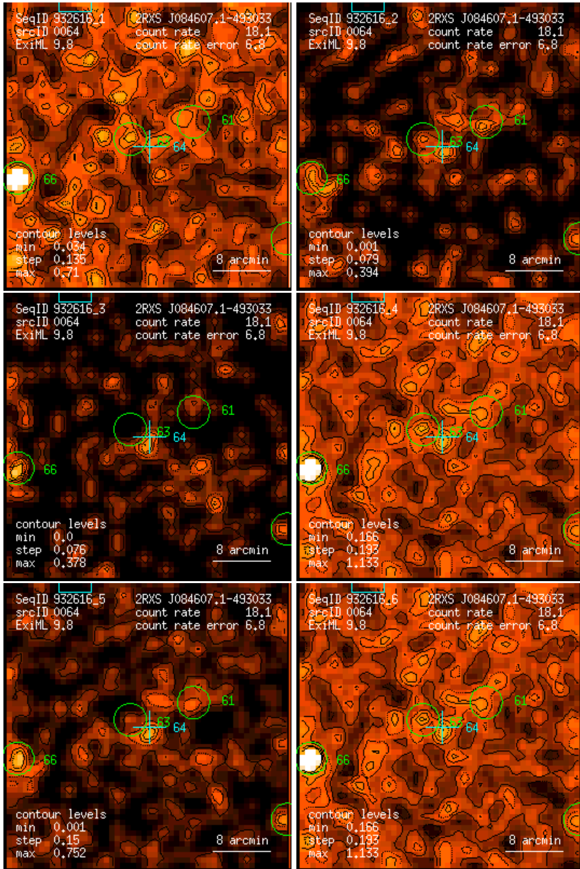
Figure 64: RASS 932616: detection 0064: band rate images, Gaussian filter: (1) PSPC channels 11 – 41, (2) 52 – 90, (3) 91 – 201, (4) 11 – 235, (5) 52 – 201, (6) 11 – 201. Broad band rates in counts/ks. Band rate contour levels in counts/ks/arcmin 2 .
