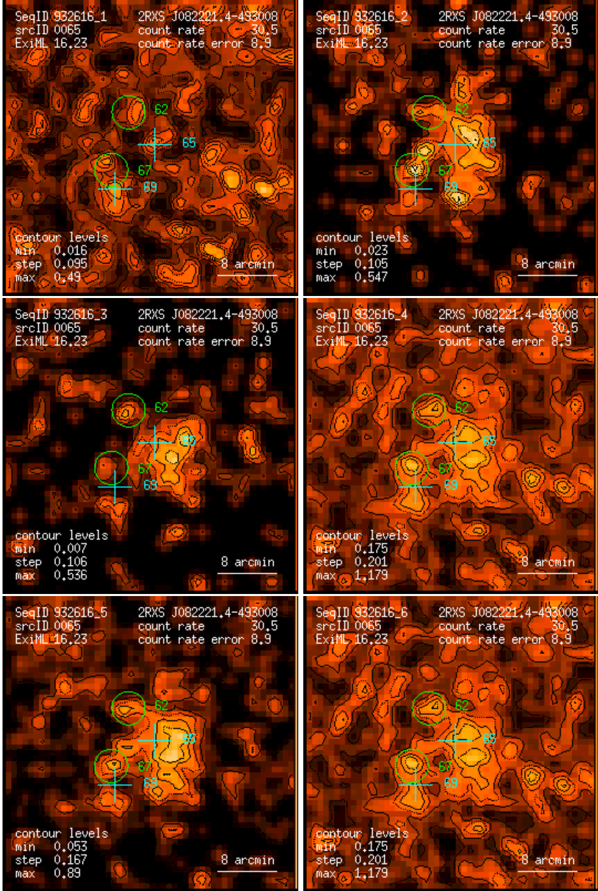
Figure 65: RASS 932616: detection 0065: band rate images, Gaussian filter: (1) PSPC channels 11 – 41, (2) 52 – 90, (3) 91 – 201, (4) 11 – 235, (5) 52 – 201, (6) 11 – 201. Broad band rates in counts/ks. Band rate contour levels in counts/ks/arcmin 2 .
