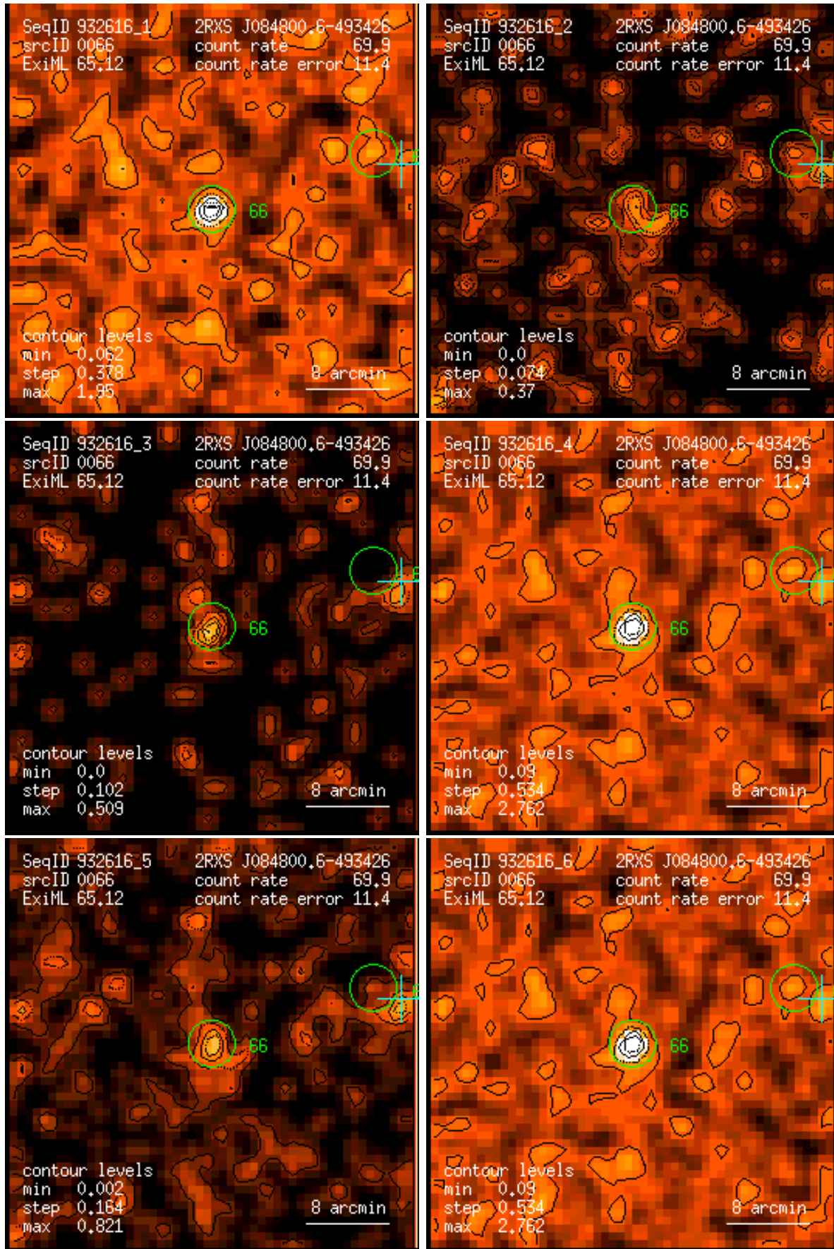
Figure 66: RASS 932616: detection 0066: band rate images, Gaussian filter: (1) PSPC channels 11 – 41, (2) 52 – 90, (3) 91 – 201, (4) 11 – 235, (5) 52 – 201, (6) 11 – 201. Broad band rates in counts/ks. Band rate contour levels in counts/ks/arcmin 2 .
