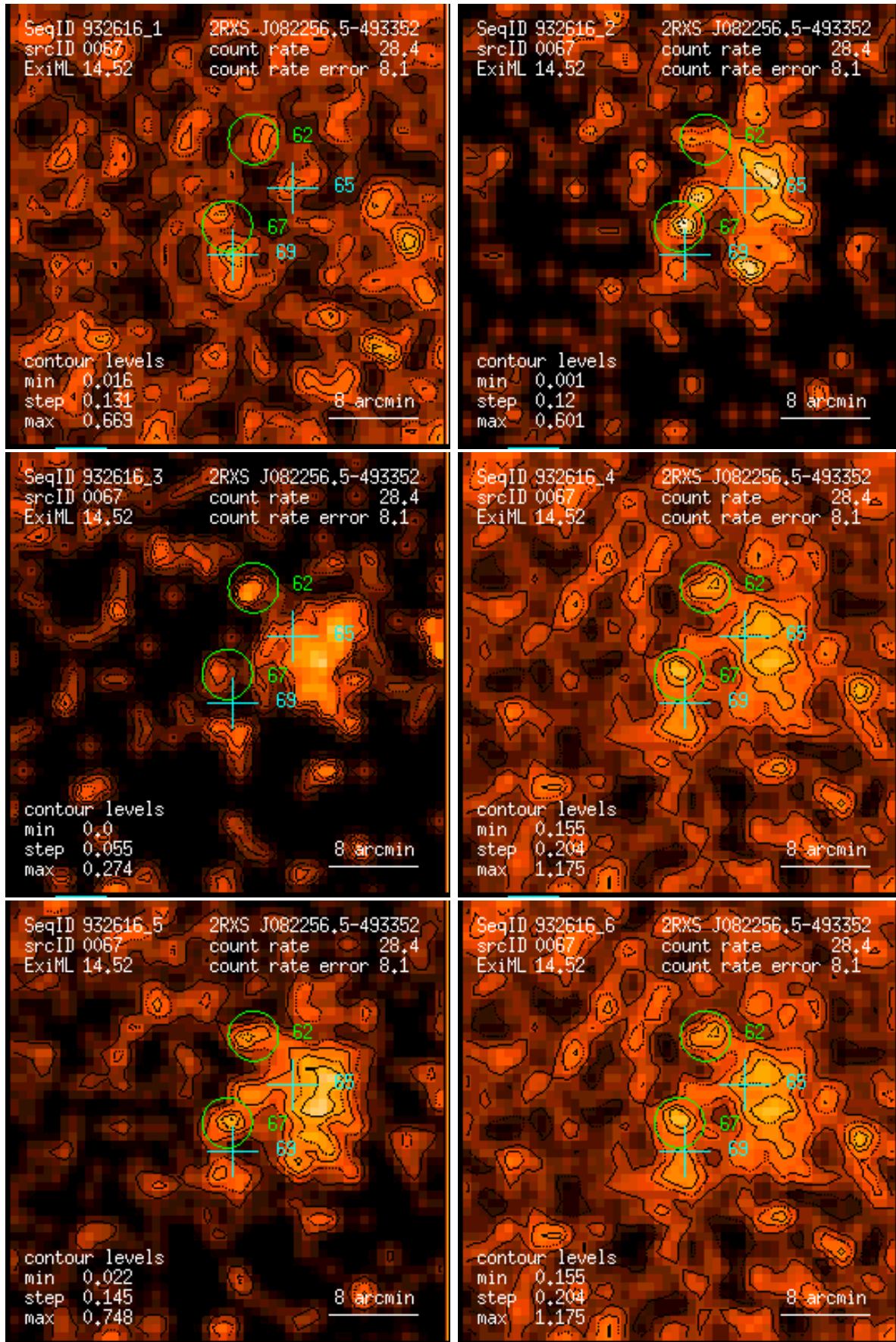
Figure 67: RASS 932616: detection 0067: band rate images, Gaussian filter: (1) PSPC channels 11 – 41, (2) 52 – 90, (3) 91 – 201, (4) 11 – 235, (5) 52 – 201, (6) 11 – 201. Broad band rates in counts/ks. Band rate contour levels in counts/ks/arcmin 2 .
