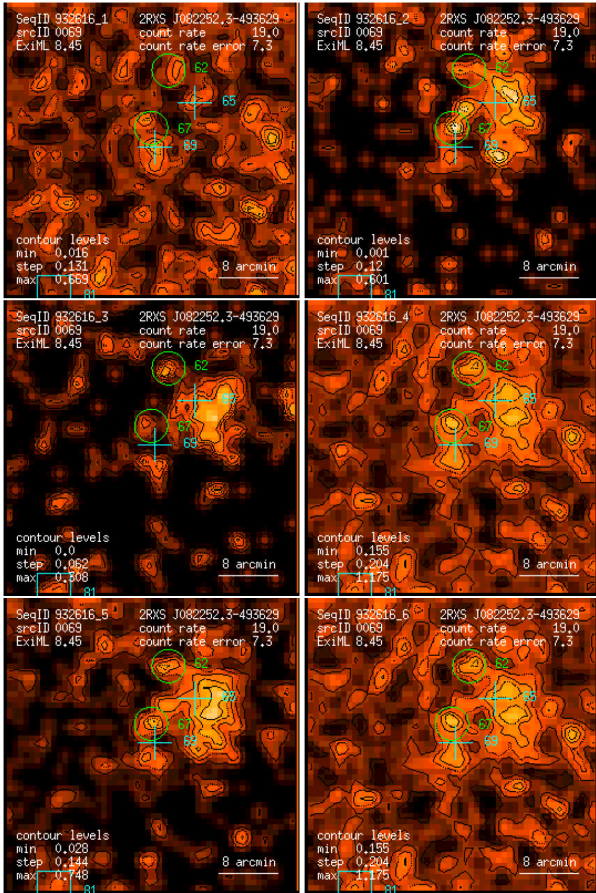
Figure 69: RASS 932616: detection 0069: band rate images, Gaussian filter: (1) PSPC channels 11 – 41, (2) 52 – 90, (3) 91 – 201, (4) 11 – 235, (5) 52 – 201, (6) 11 – 201. Broad band rates in counts/ks. Band rate contour levels in counts/ks/arcmin 2 .
