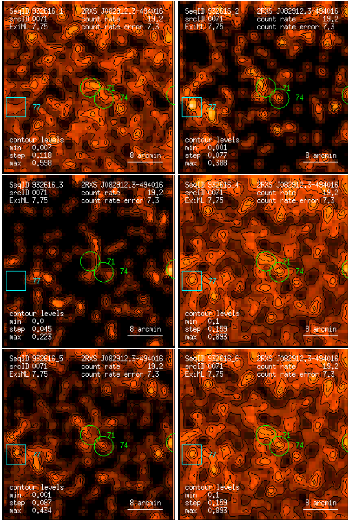
Figure 71: RASS 932616: detection 0071: band rate images, Gaussian filter: (1) PSPC channels 11 – 41, (2) 52 – 90, (3) 91 – 201, (4) 11 – 235, (5) 52 – 201, (6) 11 – 201. Broad band rates in counts/ks. Band rate contour levels in counts/ks/arcmin 2 .
