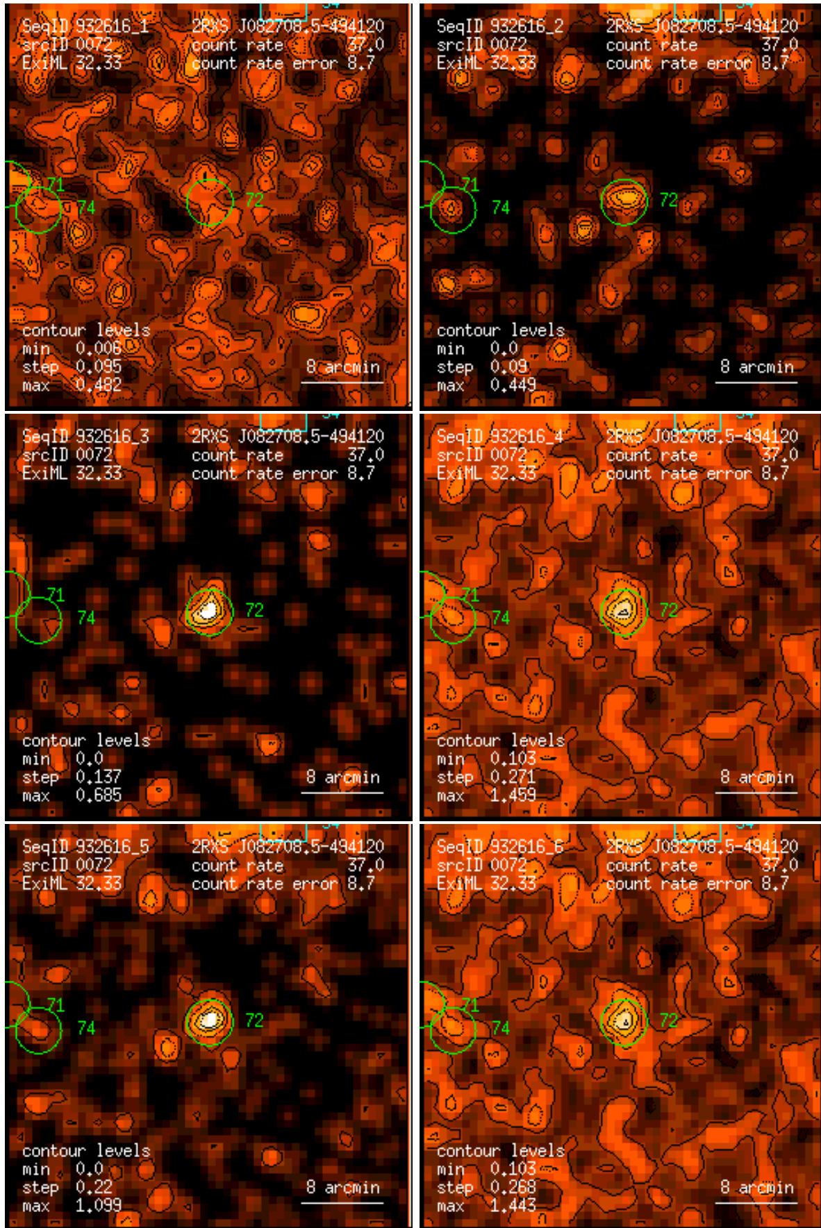
Figure 72: RASS 932616: detection 0072: band rate images, Gaussian filter: (1) PSPC channels 11 – 41, (2) 52 – 90, (3) 91 – 201, (4) 11 – 235, (5) 52 – 201, (6) 11 – 201. Broad band rates in counts/ks. Band rate contour levels in counts/ks/arcmin 2 .
