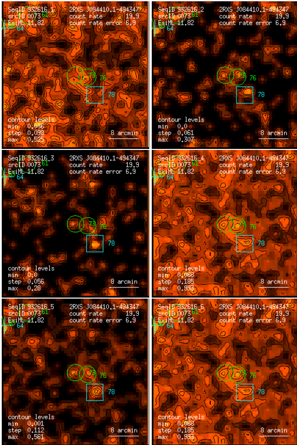
Figure 73: RASS 932616: detection 0073: band rate images, Gaussian filter: (1) PSPC channels 11 – 41, (2) 52 – 90, (3) 91 – 201, (4) 11 – 235, (5) 52 – 201, (6) 11 – 201. Broad band rates in counts/ks. Band rate contour levels in counts/ks/arcmin 2 .
