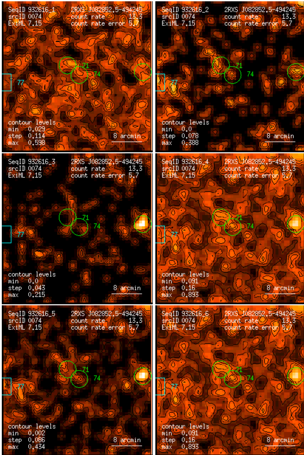
Figure 74: RASS 932616: detection 0074: band rate images, Gaussian filter: (1) PSPC channels 11 – 41, (2) 52 – 90, (3) 91 – 201, (4) 11 – 235, (5) 52 – 201, (6) 11 – 201. Broad band rates in counts/ks. Band rate contour levels in counts/ks/arcmin 2 .
