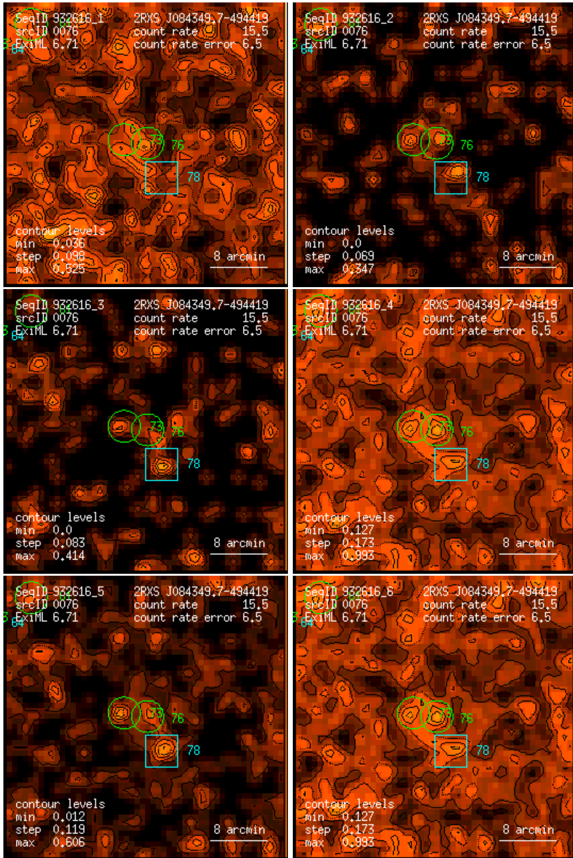
Figure 76: RASS 932616: detection 0076: band rate images, Gaussian filter: (1) PSPC channels 11 – 41, (2) 52 – 90, (3) 91 – 201, (4) 11 – 235, (5) 52 – 201, (6) 11 – 201. Broad band rates in counts/ks. Band rate contour levels in counts/ks/arcmin 2 .
