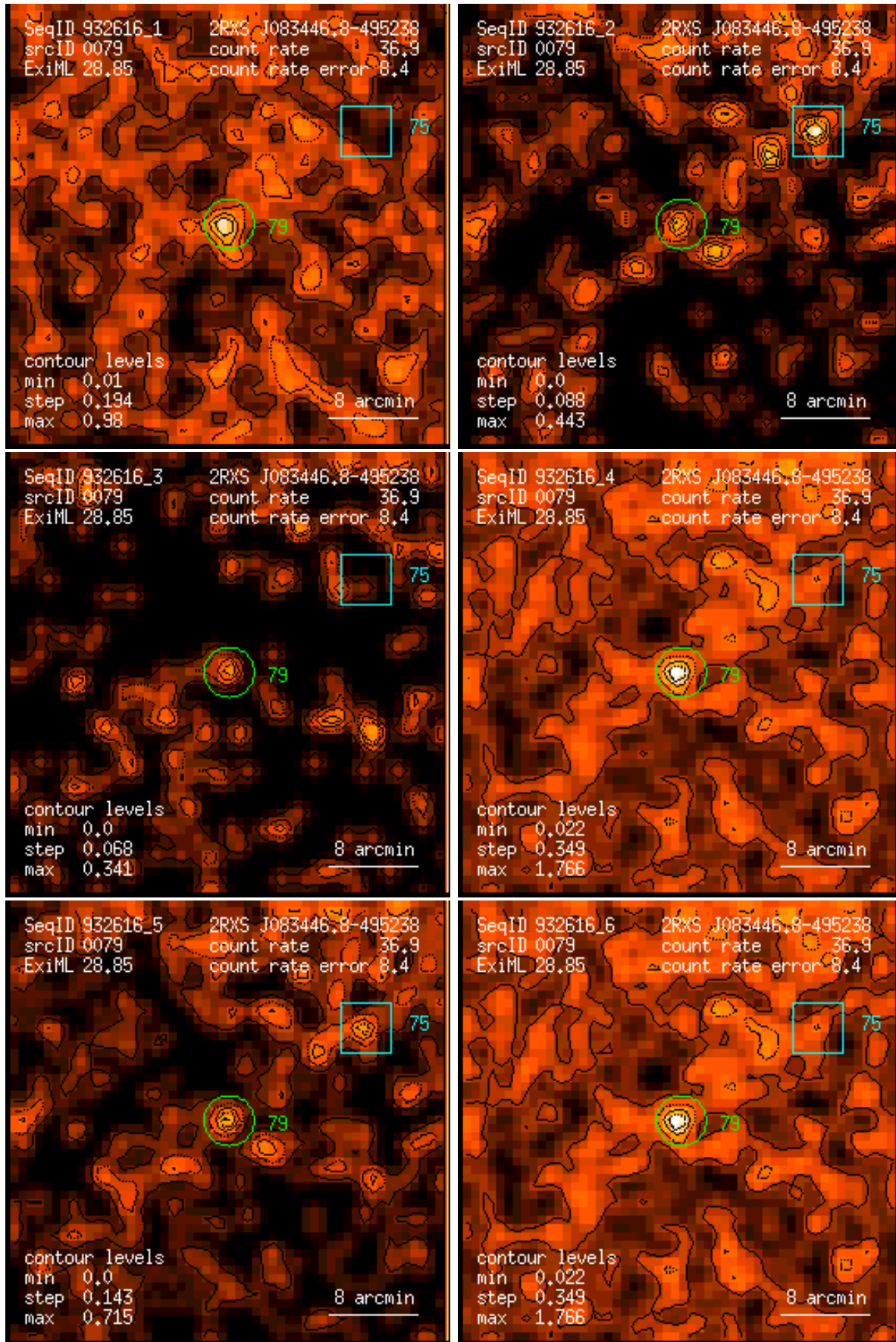
Figure 79: RASS 932616: detection 0079: band rate images, Gaussian filter: (1) PSPC channels 11 – 41, (2) 52 – 90, (3) 91 – 201, (4) 11 – 235, (5) 52 – 201, (6) 11 – 201. Broad band rates in counts/ks. Band rate contour levels in counts/ks/arcmin 2 .
