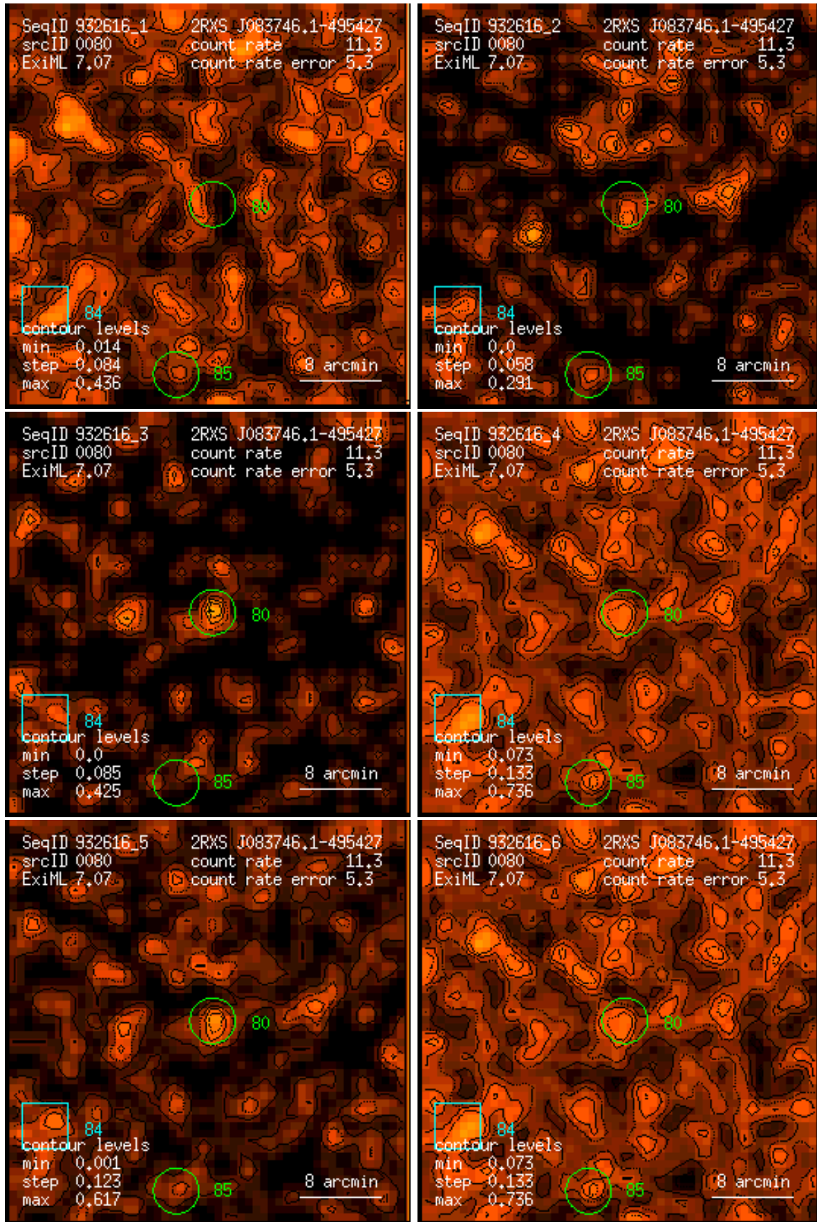
Figure 80: RASS 932616: detection 0080: band rate images, Gaussian filter: (1) PSPC channels 11 – 41, (2) 52 – 90, (3) 91 – 201, (4) 11 – 235, (5) 52 – 201, (6) 11 – 201. Broad band rates in counts/ks. Band rate contour levels in counts/ks/arcmin 2 .
