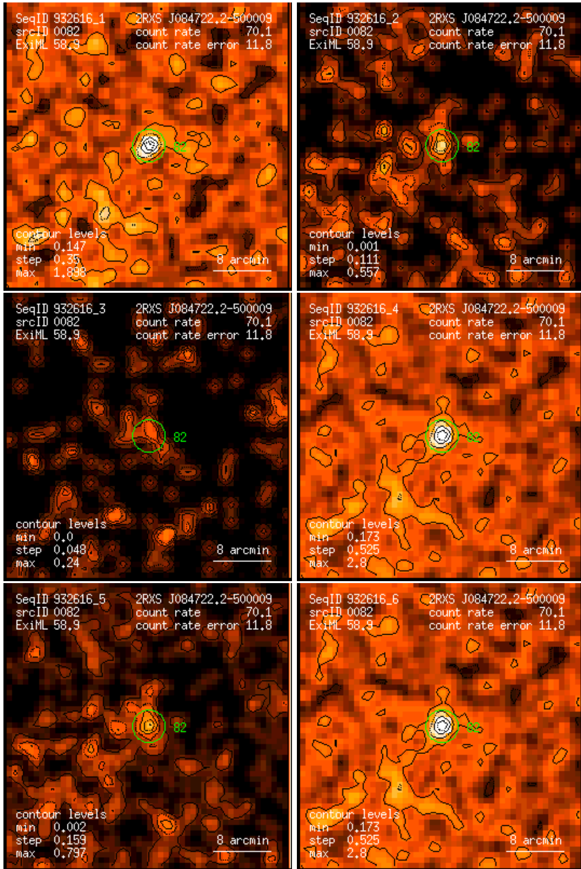
Figure 82: RASS 932616: detection 0082: band rate images, Gaussian filter: (1) PSPC channels 11 – 41, (2) 52 – 90, (3) 91 – 201, (4) 11 – 235, (5) 52 – 201, (6) 11 – 201. Broad band rates in counts/ks. Band rate contour levels in counts/ks/arcmin 2 .
