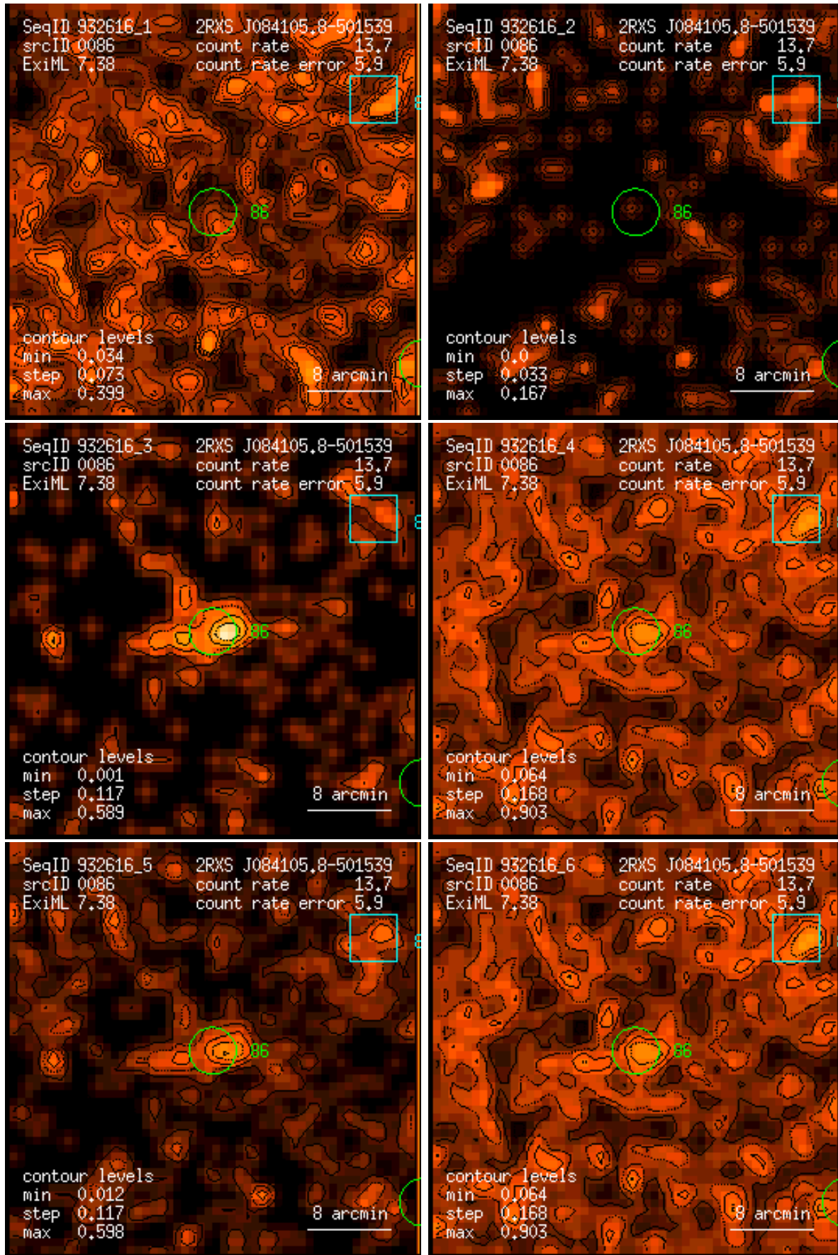
Figure 86: RASS 932616: detection 0086: band rate images, Gaussian filter: (1) PSPC channels 11 – 41, (2) 52 – 90, (3) 91 – 201, (4) 11 – 235, (5) 52 – 201, (6) 11 – 201. Broad band rates in counts/ks. Band rate contour levels in counts/ks/arcmin 2 .
