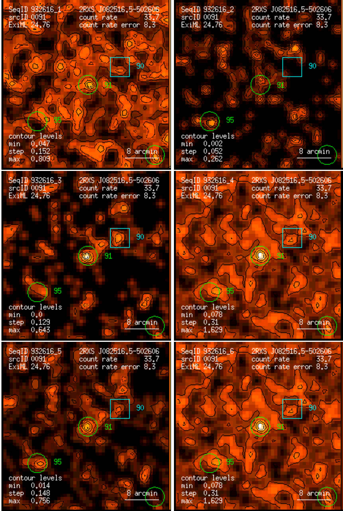
Figure 91: RASS 932616: detection 0091: band rate images, Gaussian filter: (1) PSPC channels 11 – 41, (2) 52 – 90, (3) 91 – 201, (4) 11 – 235, (5) 52 – 201, (6) 11 – 201. Broad band rates in counts/ks. Band rate contour levels in counts/ks/arcmin 2 .
