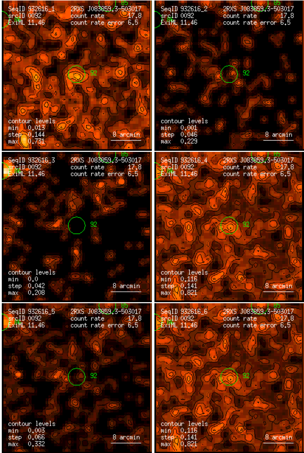
Figure 92: RASS 932616: detection 0092: band rate images, Gaussian filter: (1) PSPC channels 11 – 41, (2) 52 – 90, (3) 91 – 201, (4) 11 – 235, (5) 52 – 201, (6) 11 – 201. Broad band rates in counts/ks. Band rate contour levels in counts/ks/arcmin 2 .
