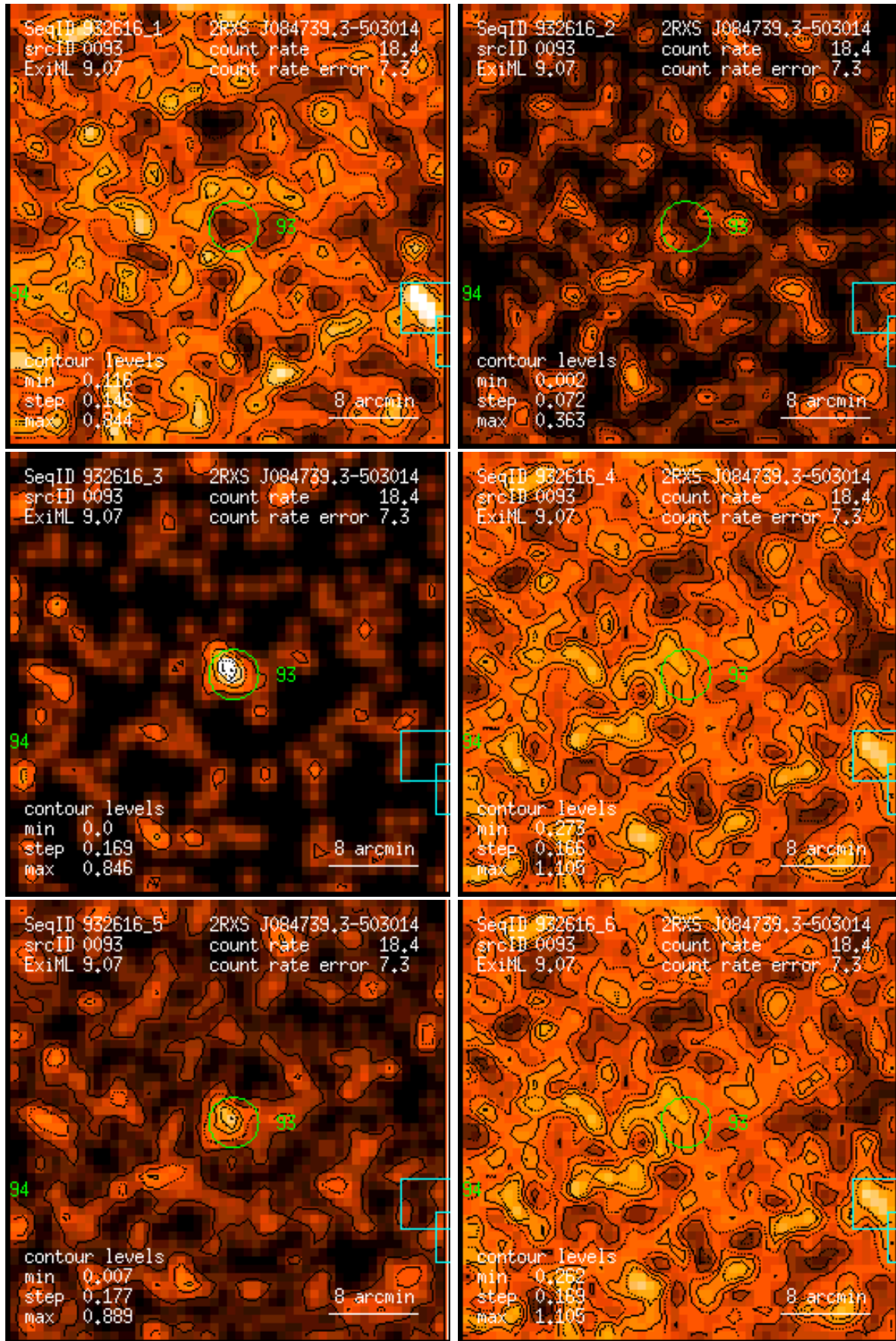
Figure 93: RASS 932616: detection 0093: band rate images, Gaussian filter: (1) PSPC channels 11 – 41, (2) 52 – 90, (3) 91 – 201, (4) 11 – 235, (5) 52 – 201, (6) 11 – 201. Broad band rates in counts/ks. Band rate contour levels in counts/ks/arcmin 2 .
