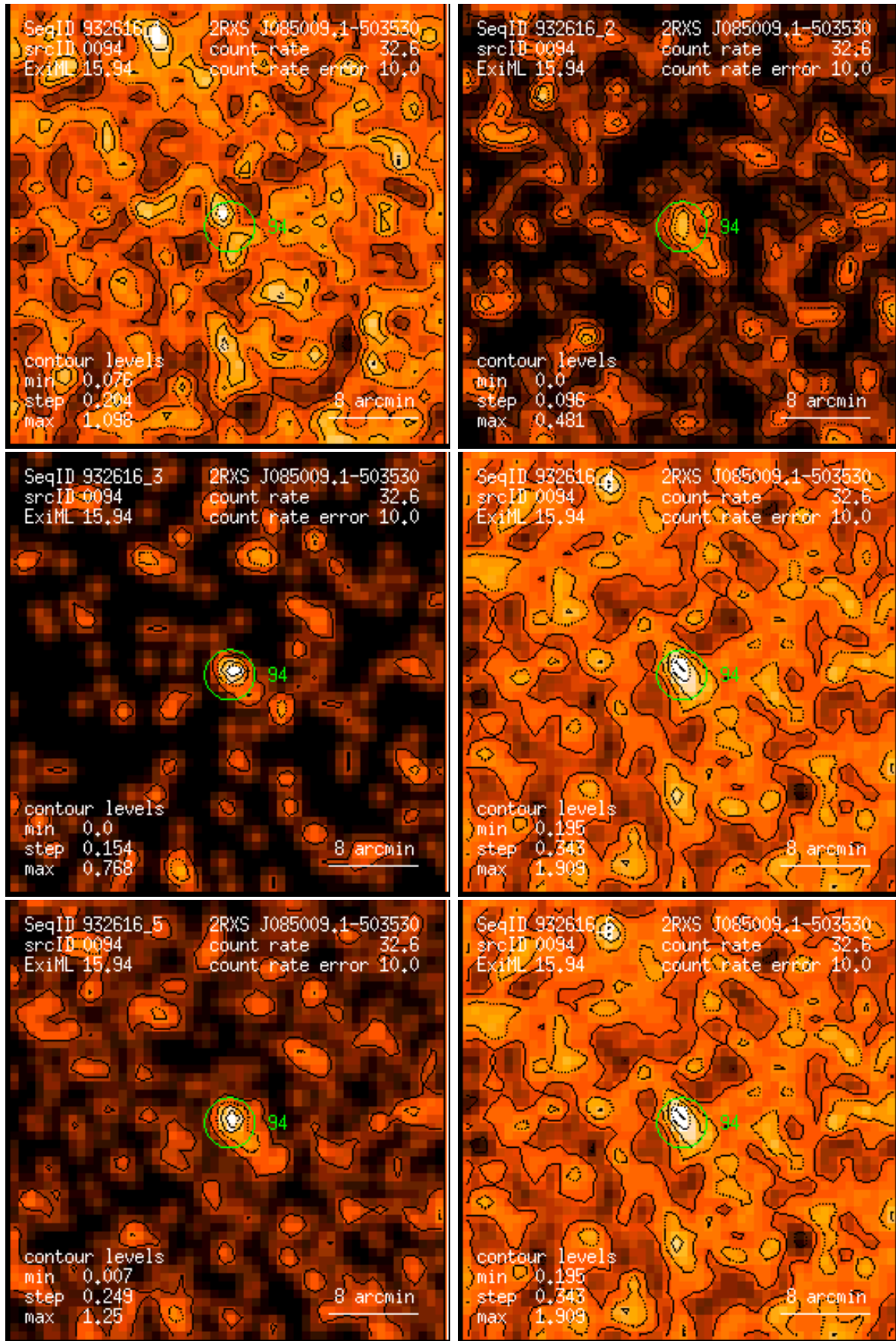
Figure 94: RASS 932616: detection 0094: band rate images, Gaussian filter: (1) PSPC channels 11 – 41, (2) 52 – 90, (3) 91 – 201, (4) 11 – 235, (5) 52 – 201, (6) 11 – 201. Broad band rates in counts/ks. Band rate contour levels in counts/ks/arcmin 2 .
