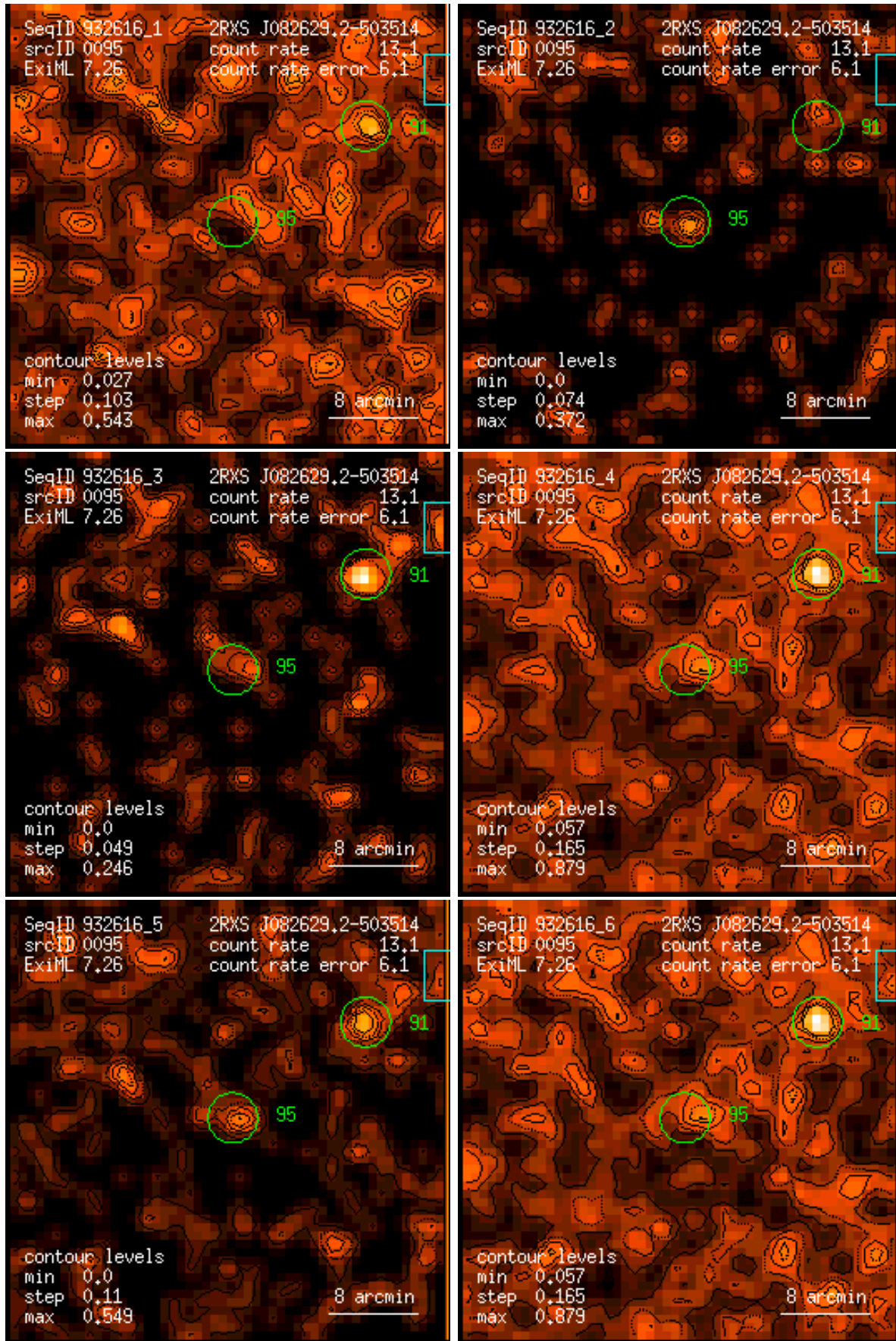
Figure 95: RASS 932616: detection 0095: band rate images, Gaussian filter: (1) PSPC channels 11 – 41, (2) 52 – 90, (3) 91 – 201, (4) 11 – 235, (5) 52 – 201, (6) 11 – 201. Broad band rates in counts/ks. Band rate contour levels in counts/ks/arcmin 2 .
