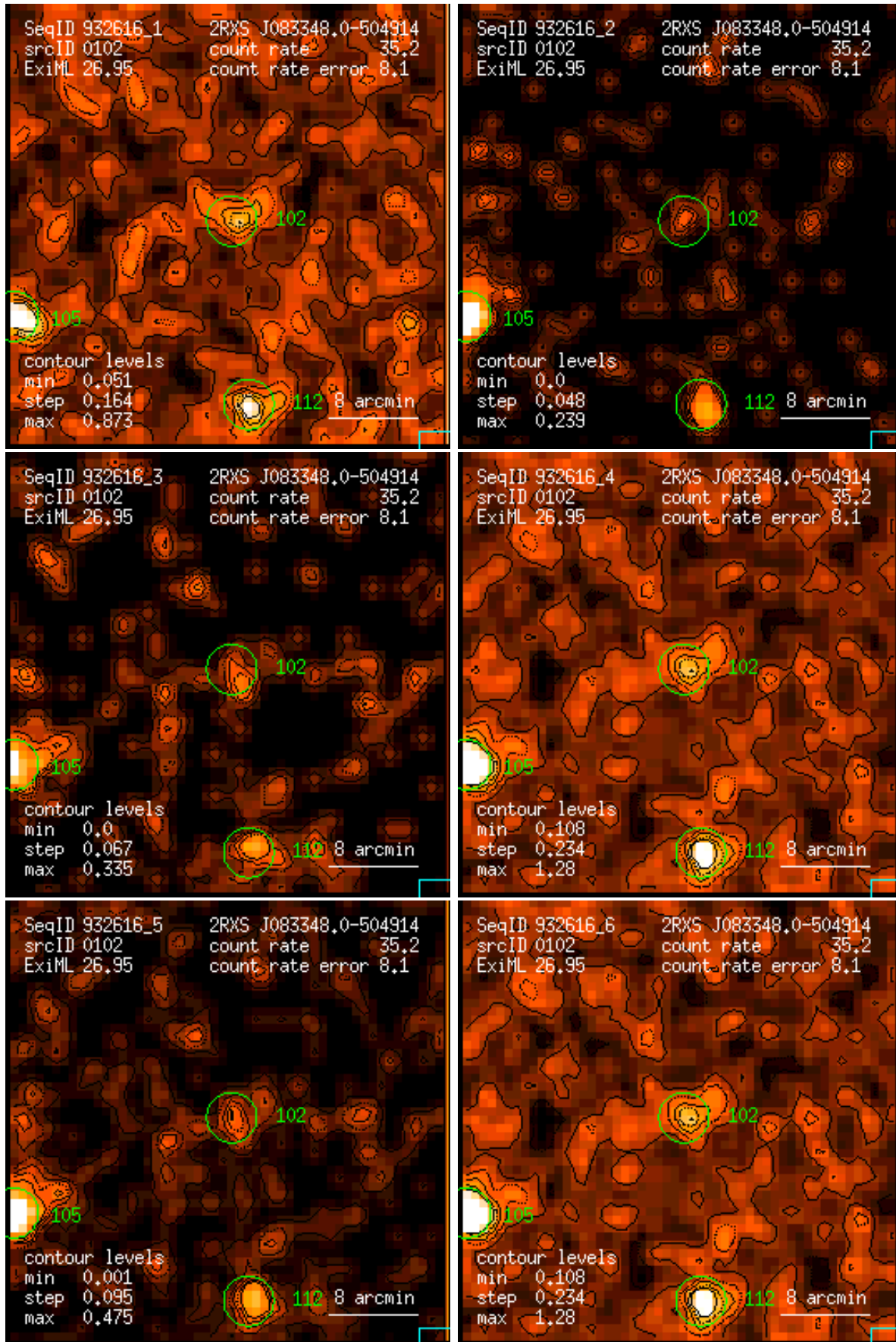
Figure 102: RASS 932616: detection 0102: band rate images, Gaussian filter: (1) PSPC channels 11 – 41, (2) 52 – 90, (3) 91 – 201, (4) 11 – 235, (5) 52 – 201, (6) 11 – 201. Broad band rates in counts/ks. Band rate contour levels in counts/ks/arcmin 2 .
