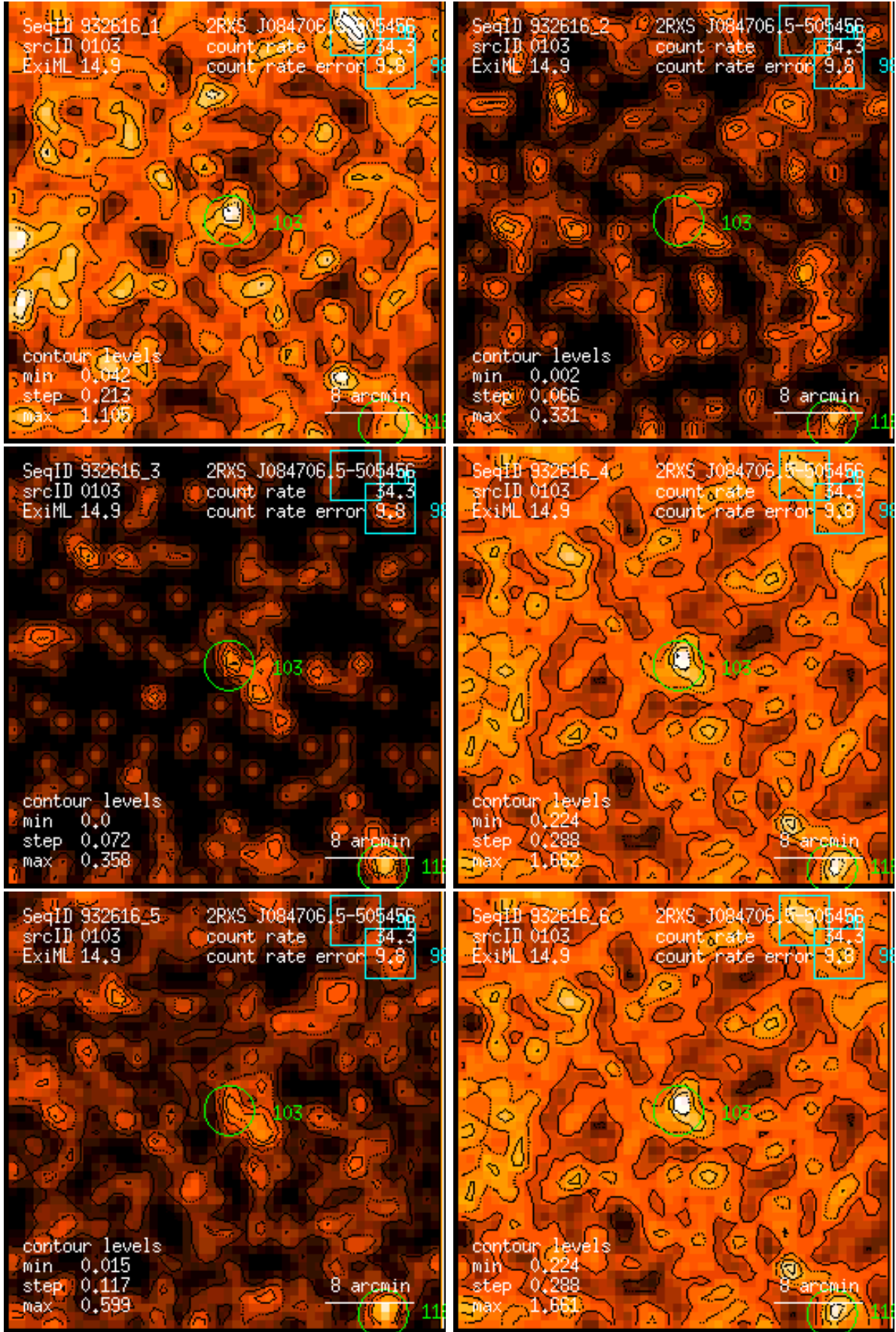
Figure 103: RASS 932616: detection 0103: band rate images, Gaussian filter: (1) PSPC channels 11 – 41, (2) 52 – 90, (3) 91 – 201, (4) 11 – 235, (5) 52 – 201, (6) 11 – 201. Broad band rates in counts/ks. Band rate contour levels in counts/ks/arcmin 2 .
