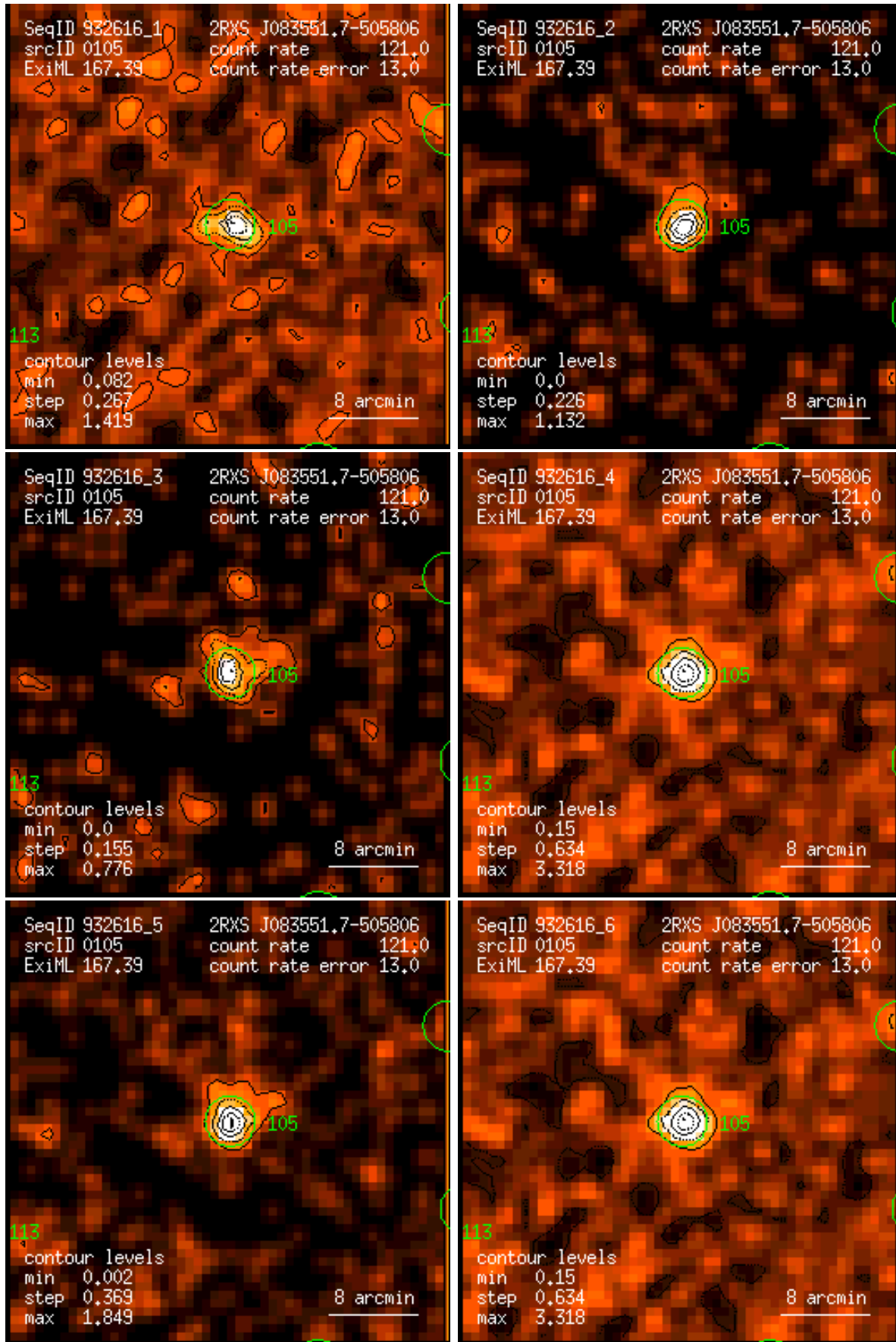
Figure 105: RASS 932616: detection 0105: band rate images, Gaussian filter: (1) PSPC channels 11 – 41, (2) 52 – 90, (3) 91 – 201, (4) 11 – 235, (5) 52 – 201, (6) 11 – 201. Broad band rates in counts/ks. Band rate contour levels in counts/ks/arcmin 2 .
