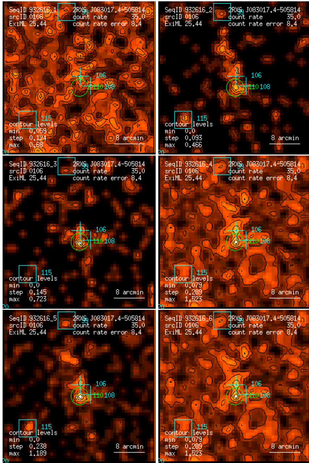
Figure 106: RASS 932616: detection 0106: band rate images, Gaussian filter: (1) PSPC channels 11 – 41, (2) 52 – 90, (3) 91 – 201, (4) 11 – 235, (5) 52 – 201, (6) 11 – 201. Broad band rates in counts/ks. Band rate contour levels in counts/ks/arcmin 2 .
