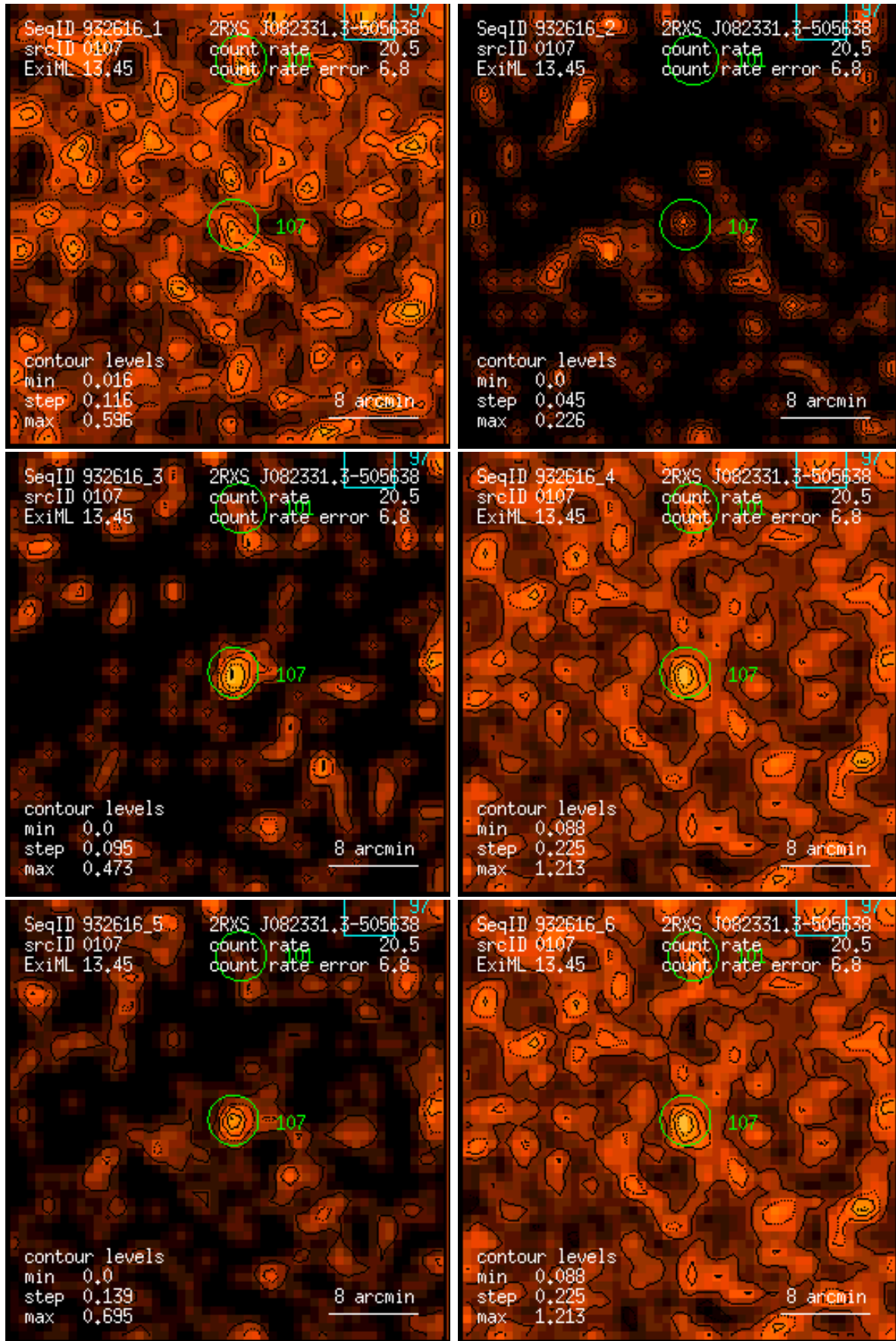
Figure 107: RASS 932616: detection 0107: band rate images, Gaussian filter: (1) PSPC channels 11 – 41, (2) 52 – 90, (3) 91 – 201, (4) 11 – 235, (5) 52 – 201, (6) 11 – 201. Broad band rates in counts/ks. Band rate contour levels in counts/ks/arcmin 2 .
