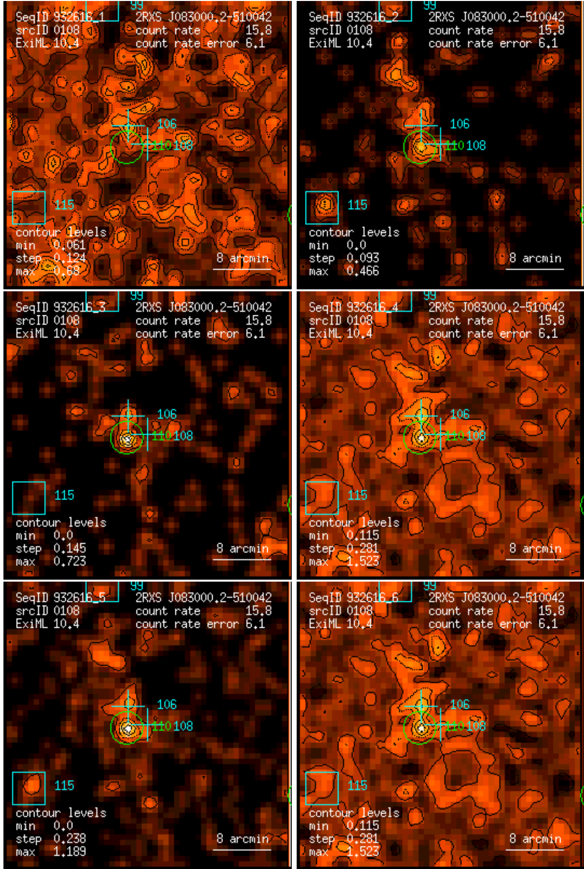
Figure 108: RASS 932616: detection 0108: band rate images, Gaussian filter: (1) PSPC channels 11 – 41, (2) 52 – 90, (3) 91 – 201, (4) 11 – 235, (5) 52 – 201, (6) 11 – 201. Broad band rates in counts/ks. Band rate contour levels in counts/ks/arcmin 2 .
